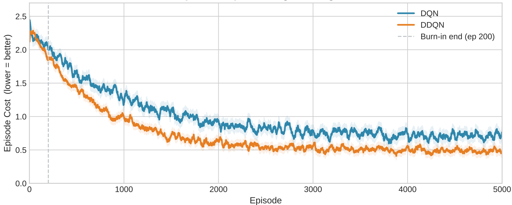
DQN vs DDQN Training Convergence
