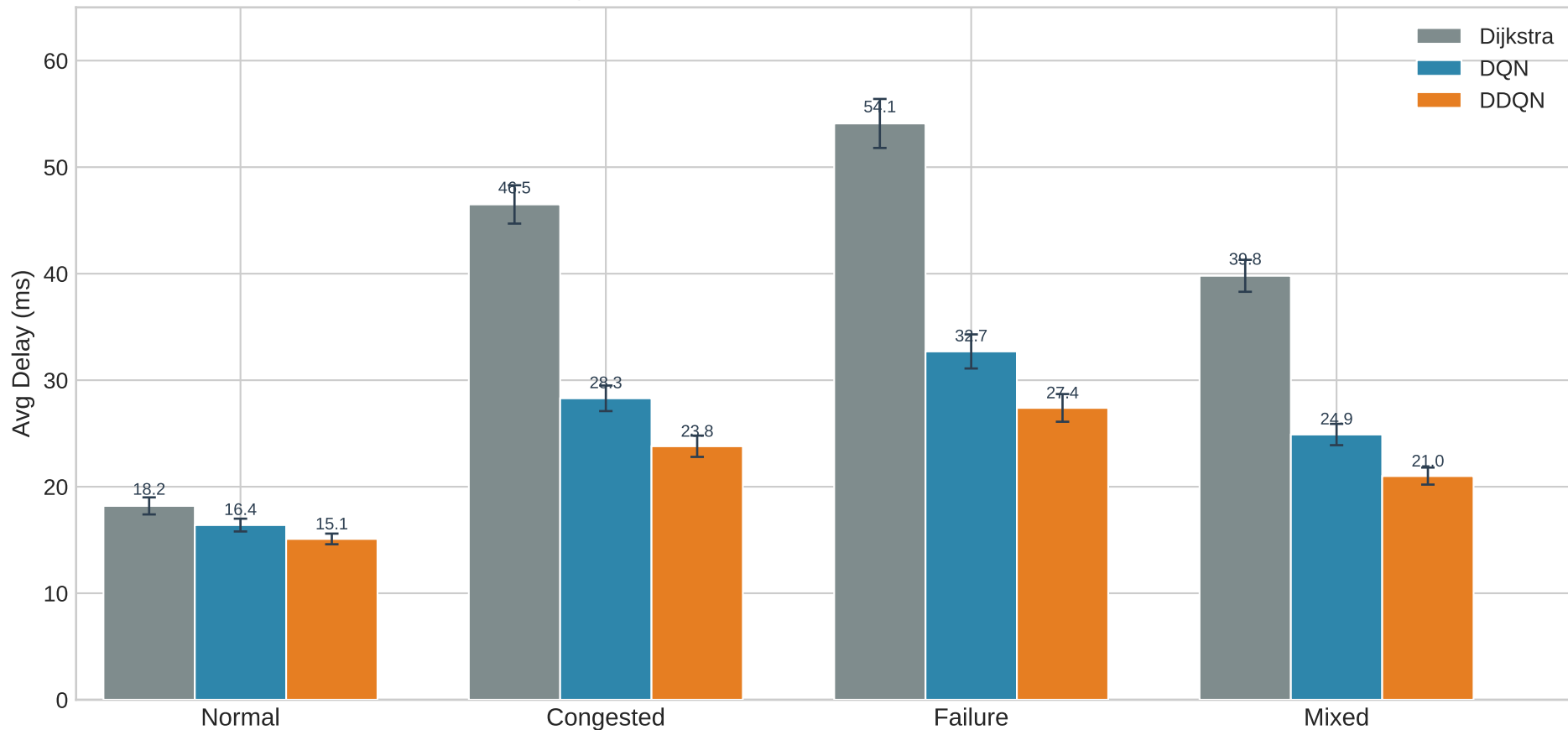
Avg Delay (ms): Dijkstra vs DQN vs DDQN
