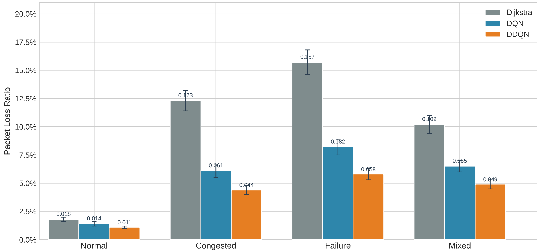
Packet Loss Ratio: Dijkstra vs DQN vs DDQN
