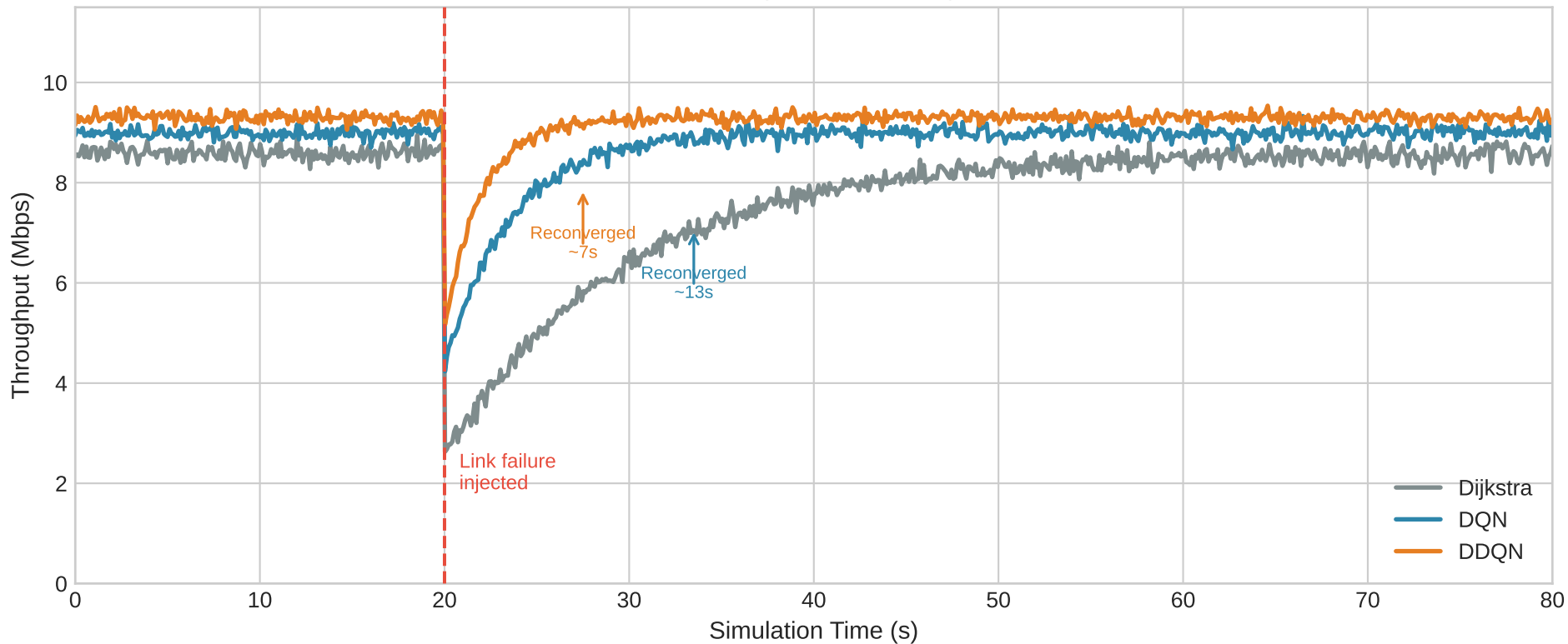
Link Failure Reconvergence: Throughput Over Time
