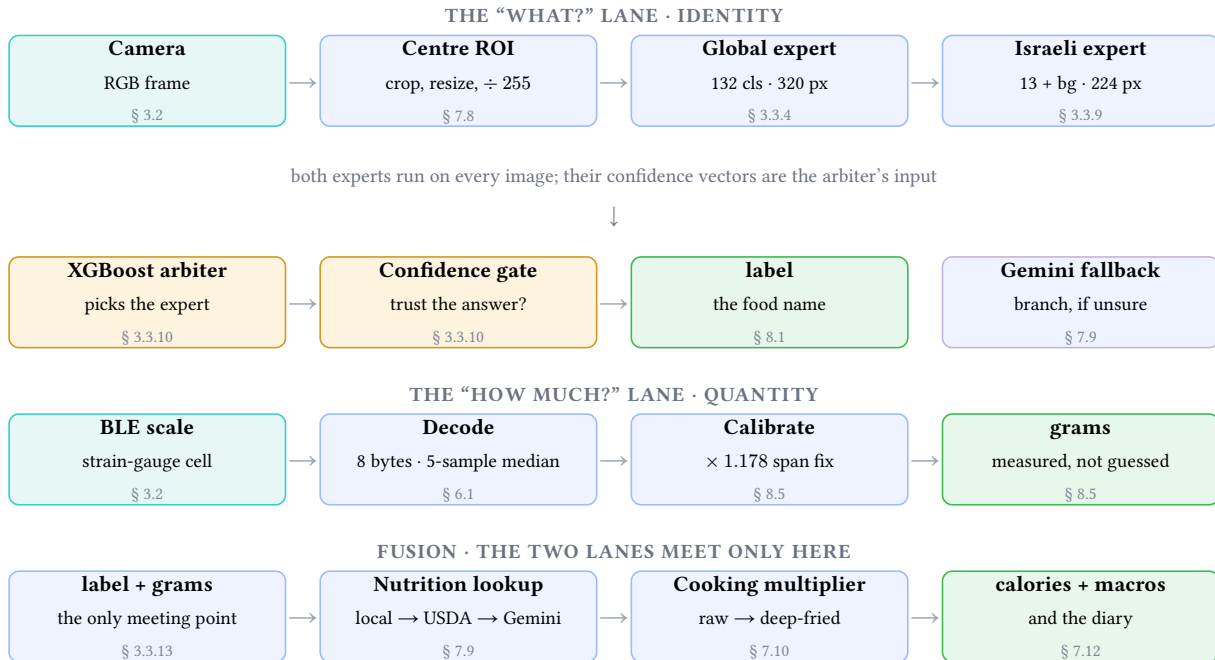
Figure 1: Roadmap: the system, and where each part of it is documented. Read this once and the rest of the book has somewhere to hang. The upper lane turns a frame into a label ; the middle lane turns a BLE packet into grams ; the two stay completely independent until the final multiplication at the bottom, which is the thesis of the project: nothing ever infers mass from pixels. Teal = a physical sensor, blue = computation, amber = the routing decision, green = a finished quantity. Each box names the section that derives it, so any stage can be read alone.
