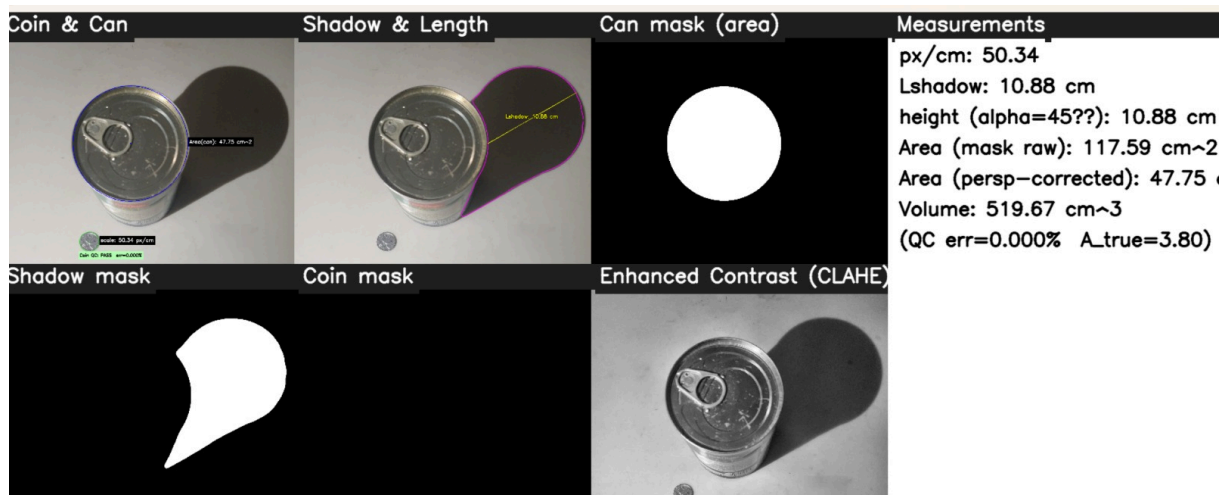
Figure 22: Volume from shadow geometry. With a 45° light an object's height equals its shadow length; the perspective-corrected top area times that height gives 519.67 cm 3 , again without any depth network - and again stuck at the density step.
