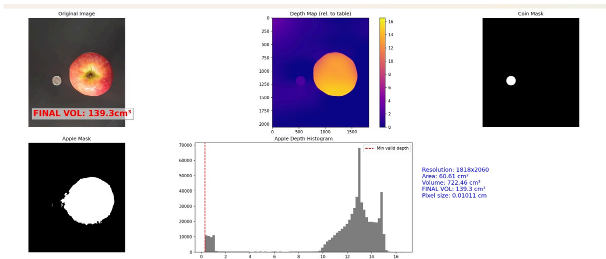
Figure 21: Volume from monocular depth (MiDaS). The coin fiducial sets pixel size; the depth map over the apple mask integrates to a volume of 139.3 cm 3 , within 7% of the true volume - yet still useless without a density value to convert it to grams.
