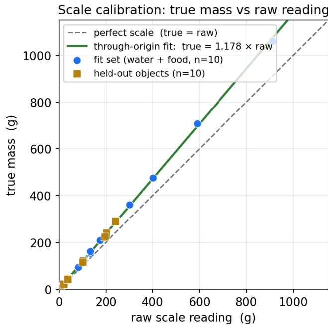
Figure 13: True mass vs raw reading. Blue = fit set (water + food, n = 10 ); amber squares = held-out everyday objects ( n = 10 ). All points lie on one through-origin line, well above the dashed perfect-scale diagonal - a constant proportional under-read, not a random or additive one.
