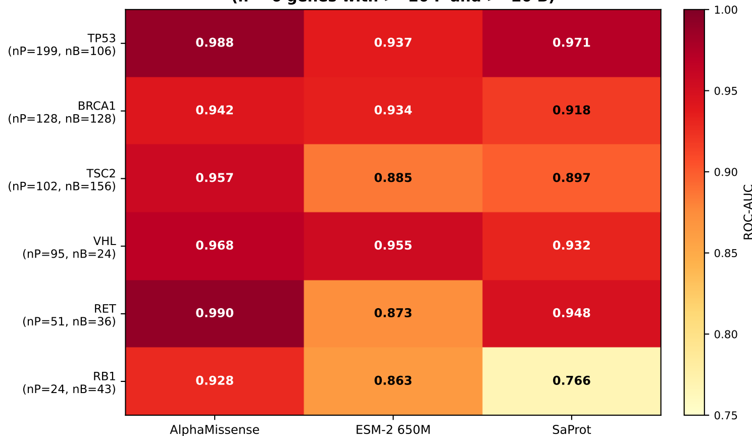
Per-gene ROC-AUC on post-AM variants (n = 6 genes with >=20 P and >=20 B)
