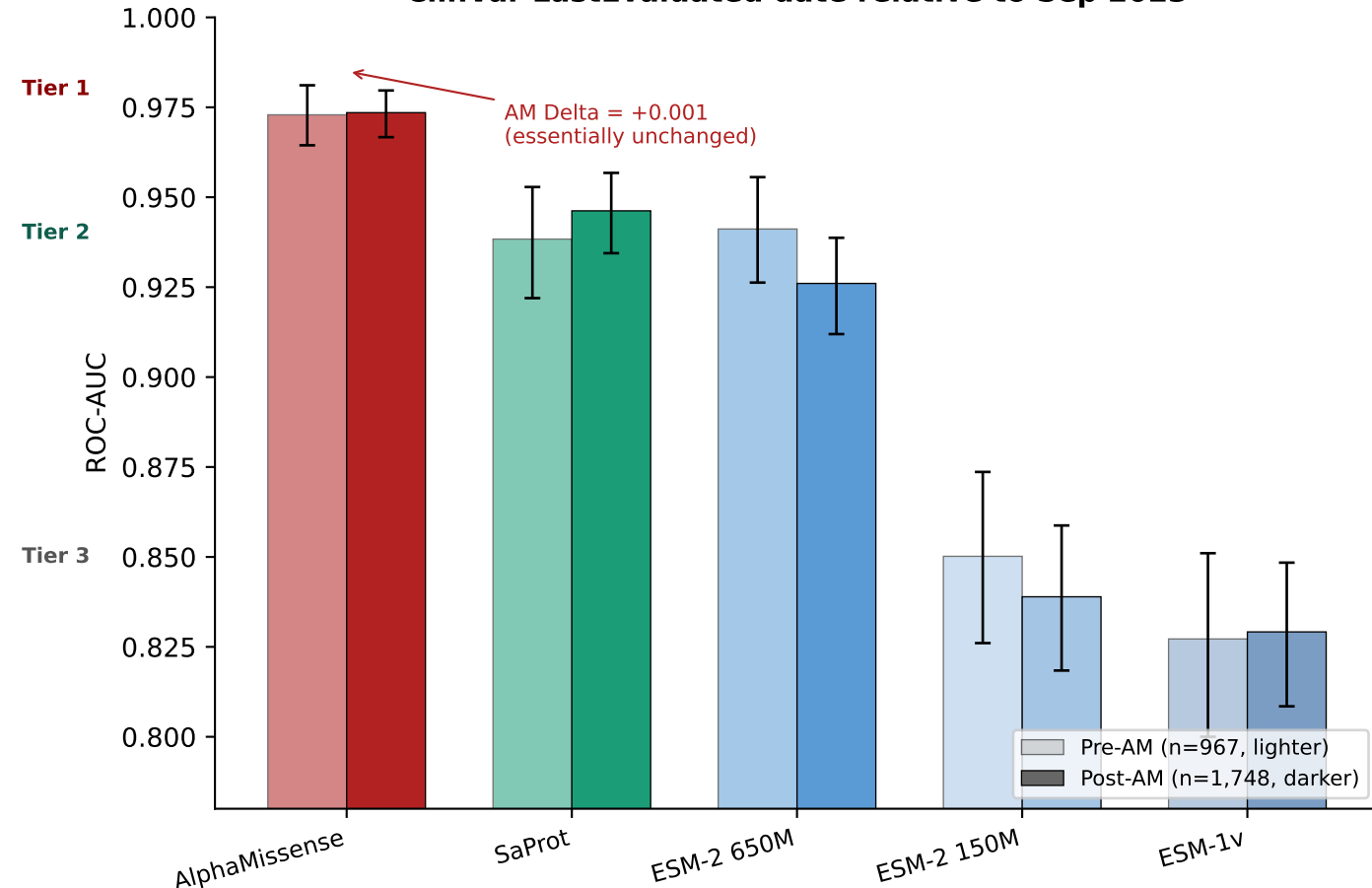
Performance stability: variants stratified by ClinVar LastEvaluated date relative to Sep 2023
