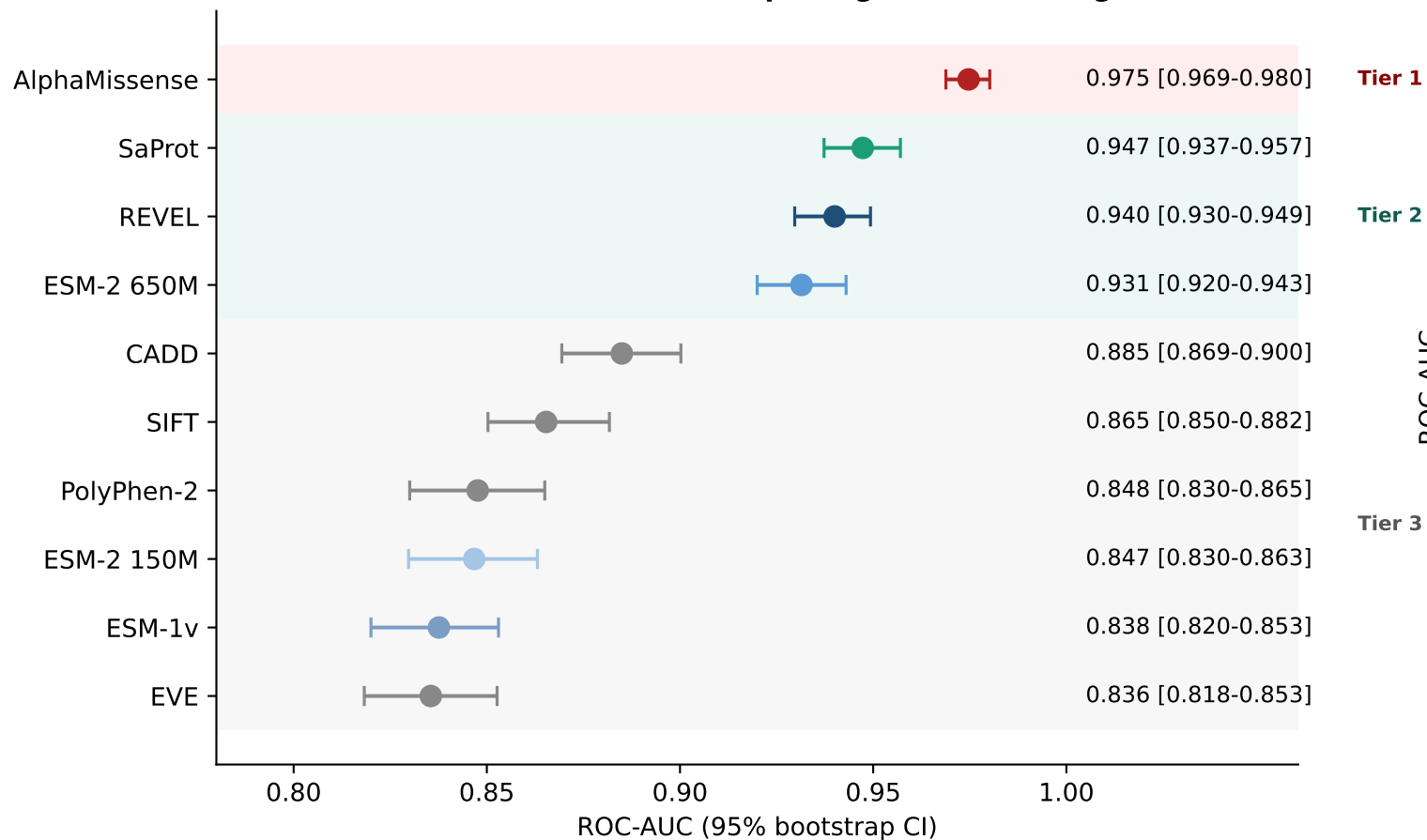
Benchmark performance: 10 methods on fully-shared subset (n = 2080 variants; 1227 pathogenic, 853 benign)
