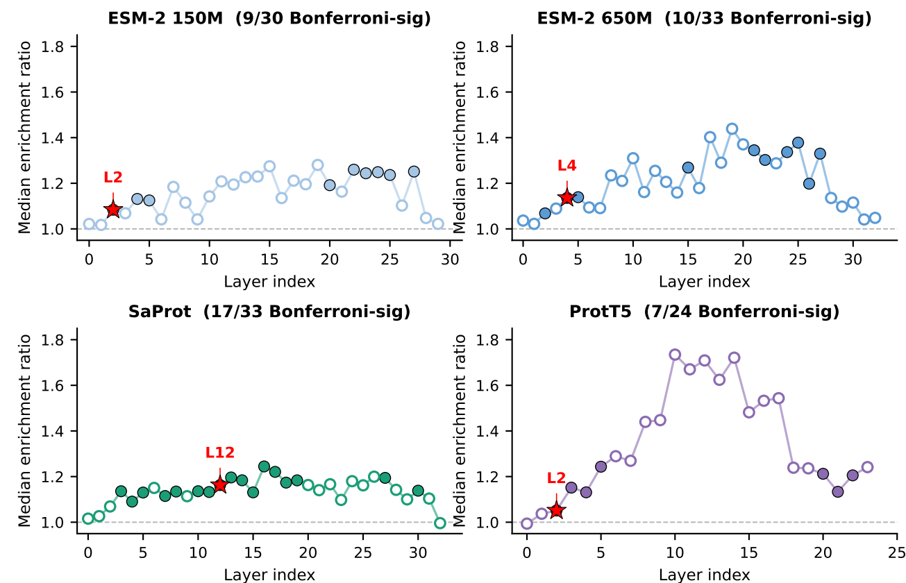
Layer-resolved attention enrichment at pathogenic sites (n = 18 proteins, conservation-matched controls)
