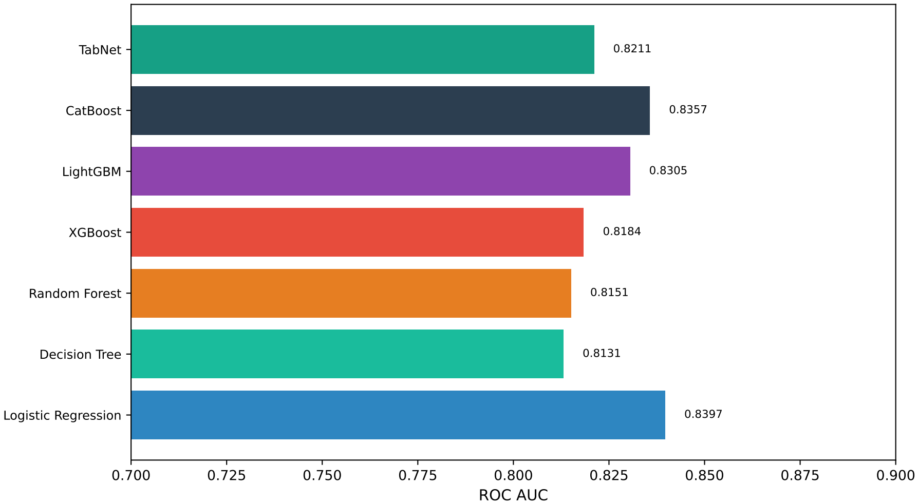
Model Performance Comparison (Telco Dataset)
