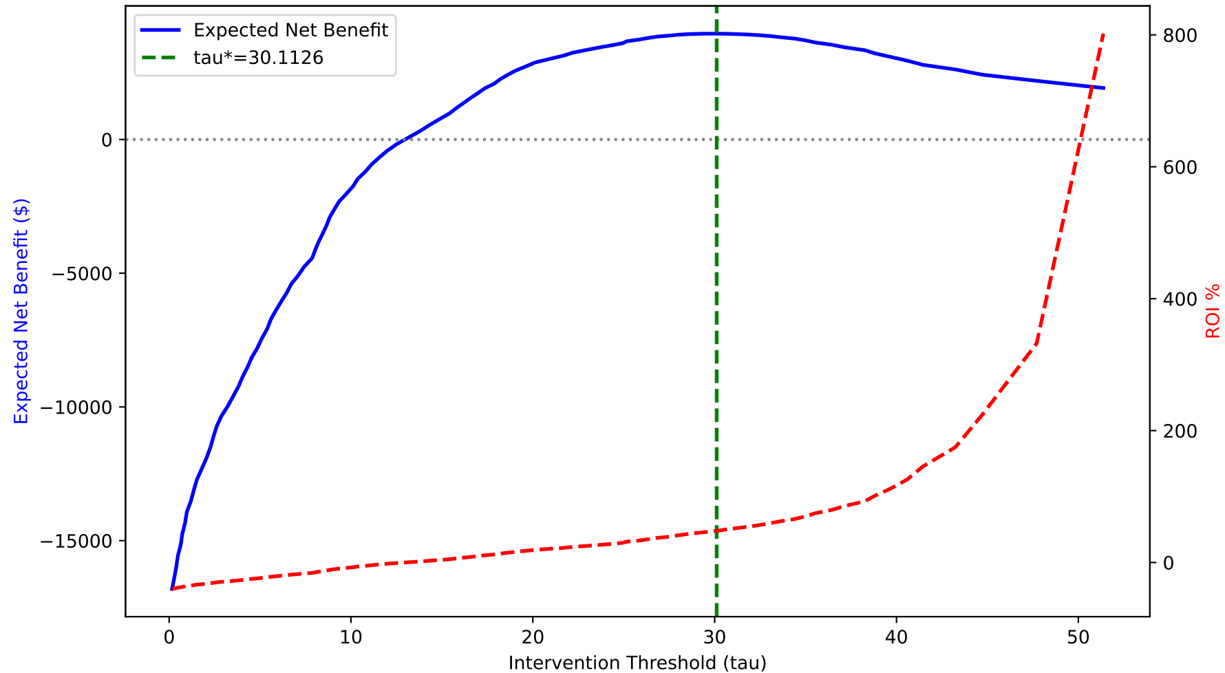
Adaptive Intervention Optimization: Expected Profit vs Threshold
