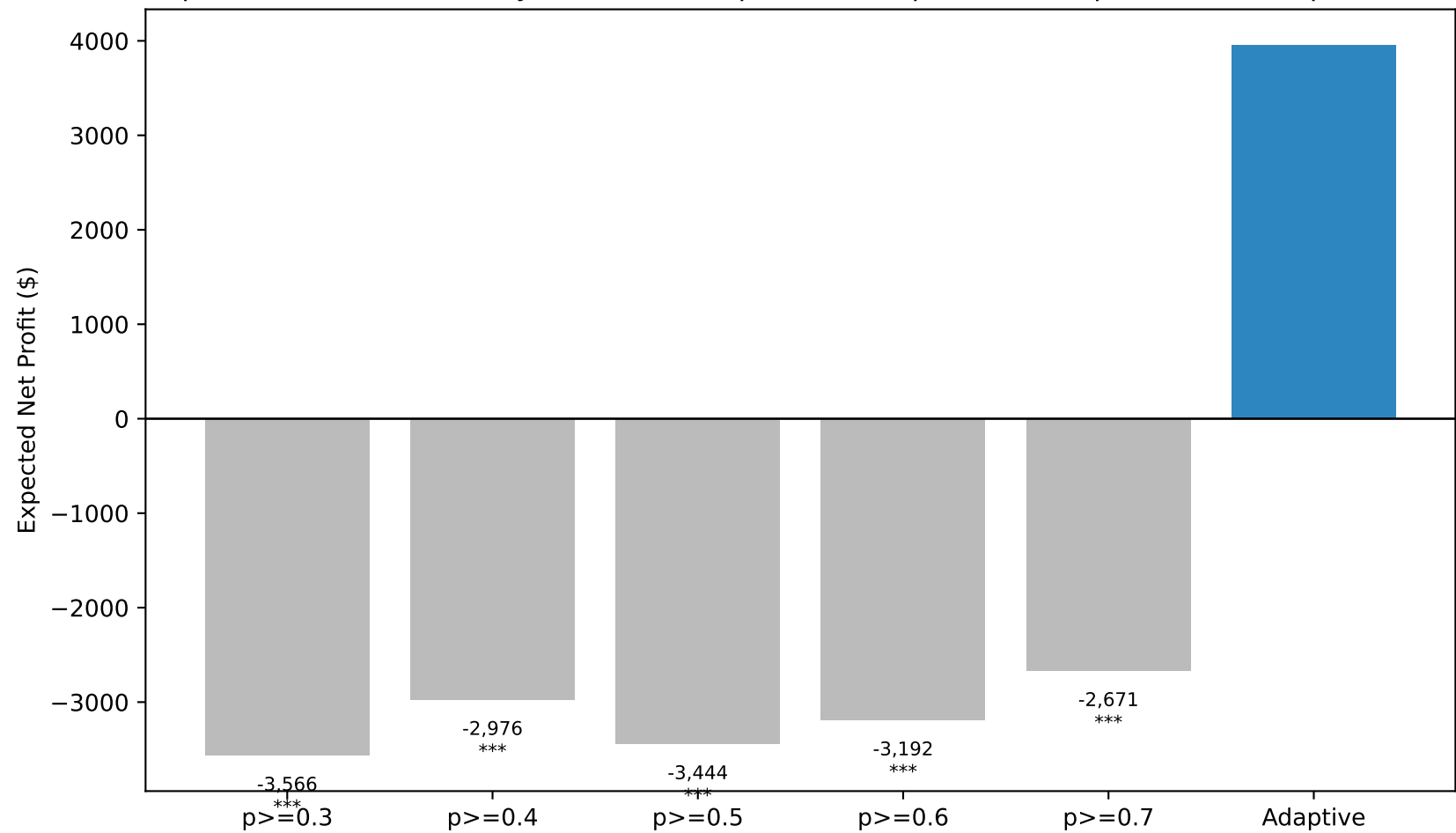
Adaptive vs Fixed Probability Thresholds (* p < 0.05 , *** p < 0.001 via paired bootstrap Wilcoxon)
