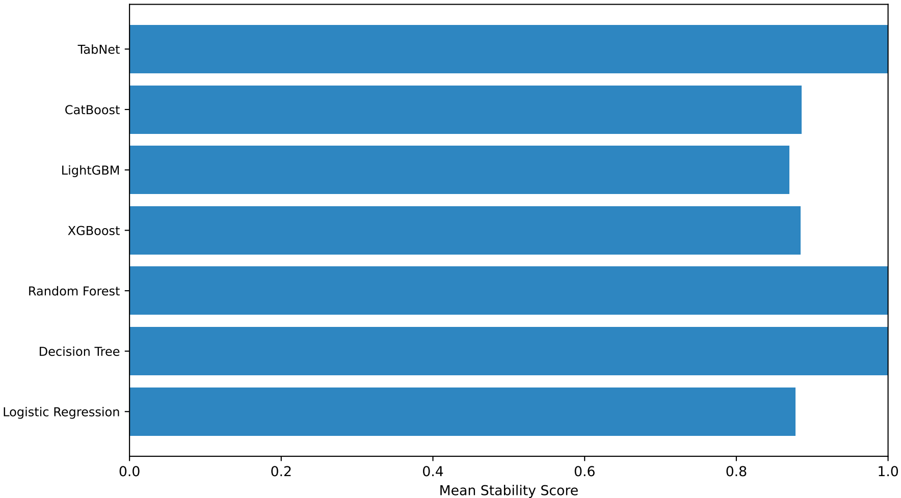
Explanation Stability Across Models
