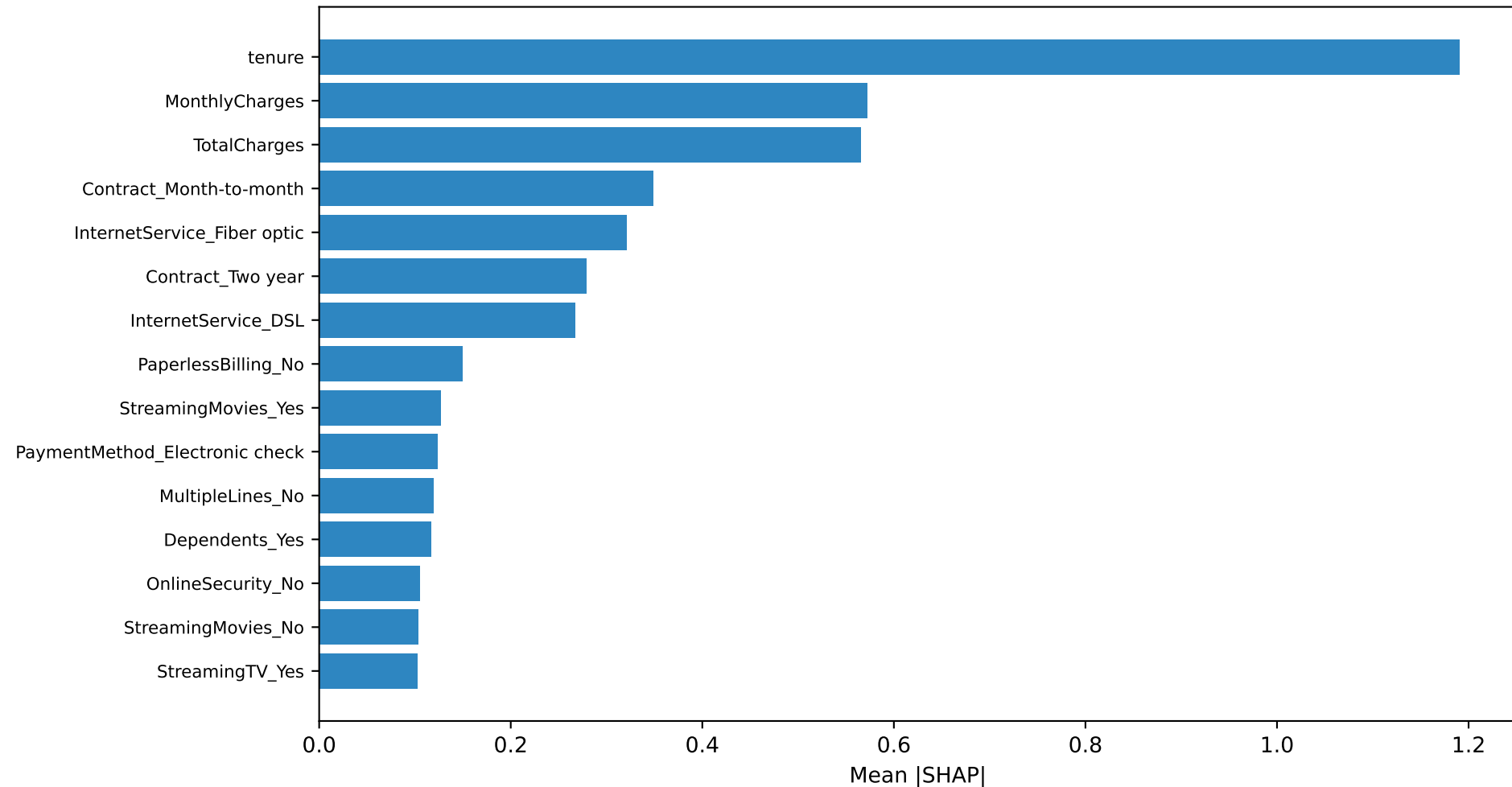
SHAP Feature Importance (Logistic Regression)
