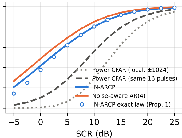
Pfa design 0.001
