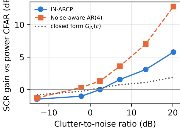
Detection, Pfa 0.01, Pd 0.5
