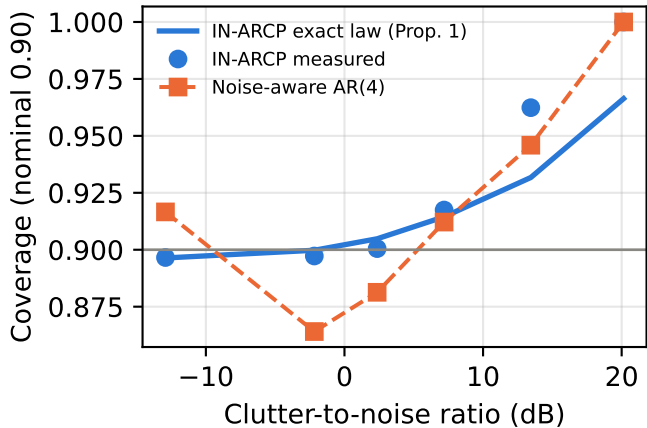
77 GHz FMCW ground clutter
