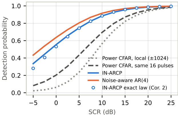
IPIX sea clutter, P_{fa} design 0.01
