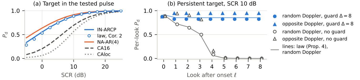
Fig. 3. Detection of Swerling-1 targets injected into IPIX test episodes ( m = 16 , conformal thresholds, per-look P_{fa} = 0.01 ). (a) Target in the tested pulse (74,980 episodes in total). NA-AR(4): noise-aware score, 8.0 dB less SCR than CA16. Circles: law of Corollary 2, model fitted on each unit's training third. Curves average P_d over units; the text averages per-unit gains. (b) Persistent 10 dB target (56 units) without and with an eight-pulse guard, markers offset for visibility; means in the text are over looks 1–8. Lines: law of Proposition 4 at the fitted AR(1) coefficient, random Doppler (exploratory).
