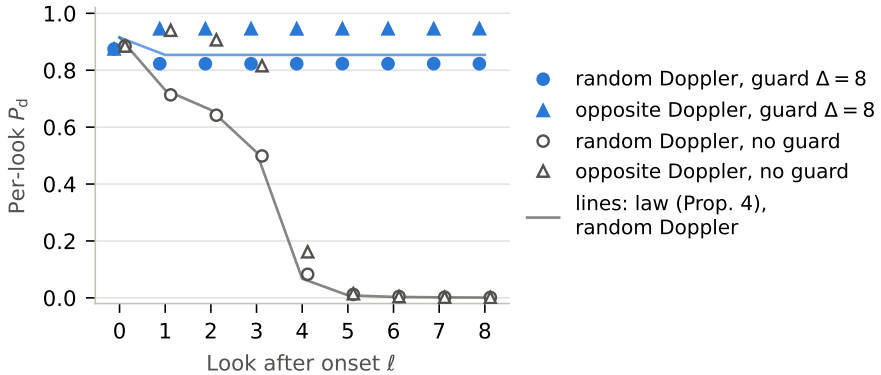
(b) Persistent target, SCR 10 dB
