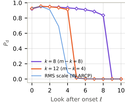
(f) Certified integration, pulsed interference
