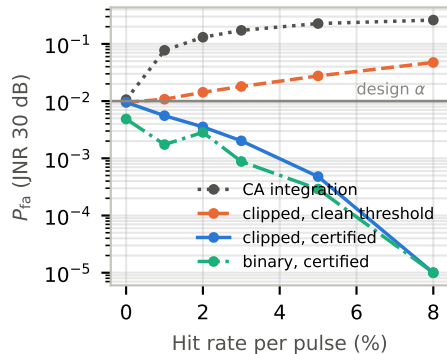
(f) Certified integration, pulsed interference
