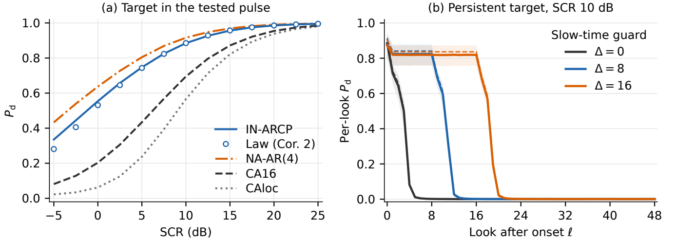
Fig. 3. Detection of Swerling-1 targets injected into IPIX test episodes ( m = 16 , conformal thresholds, design per-look P_{fa} = 0.01 ). (a) Target in the tested pulse (74,980 episodes in total). NA-AR(4): noise-aware score, 8.0 dB less SCR than CA16. Circles: law of Corollary 2, model fitted on each unit’s training third. Empirical and law curves are unit means; the text averages per-unit gains. (b) Persistent target at 10 dB SCR, random Doppler (56 units, 236,440 episodes), with guards \Delta = 0, 8, 16 , through 48 looks. Solid: episode-weighted measured P_d ; dashed: episode-weighted law of Proposition 4 at fitted AR(1) coefficients and actual thresholds (exploratory); shading: 95% day-cluster intervals.
