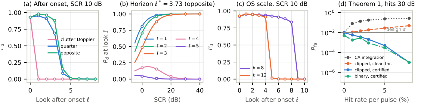
Fig. 2. Closed forms (lines) against Monte Carlo (markers; 10^5 episodes per point, 5 \times 10^4 in (b)) at the true coefficient, AR(1) compound-Gaussian clutter with \rho = 0.93e^{-0.2j} , lognormal texture, m = 16 , P_{fa} = 0.01 . (a) Proposition 4; (b) horizon, Corollary 4; (c) OS scales (quadrature); (d) Theorem 1, P_{fa} against the hit rate for Gaussian interference 30 dB above the local power (few events below 10^{-4} ). Other laws: Supplementary Material.
