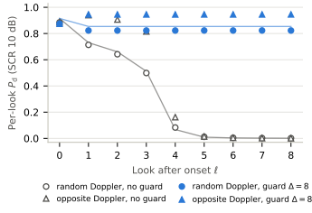
Fig. 4. Per-look detection probability after the onset of a persistent Swerling-1 target on IPIX (SCR 10 dB, per-look P_{fa} 0.01, 56 units), without and with a guard of eight pulses. Markers: measured; lines: law of Proposition 4 at the fitted AR(1) coefficient, random Doppler (exploratory).
