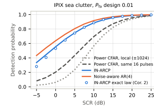
Fig. 3. Detection of Swerling-1 targets that appear in the tested pulse, injected into 74,980 IPIX test episodes ( m = 16 , conformal thresholds at design P_{fa} = 0.01 ). Power CFAR: CA16 and CALoc (Section V). Circles: exact law of Corollary 2 with the clutter-plus-noise model fitted on each unit's training third.
