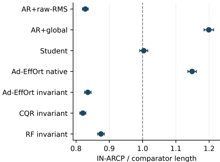
Gaussian AR(1), m=4
