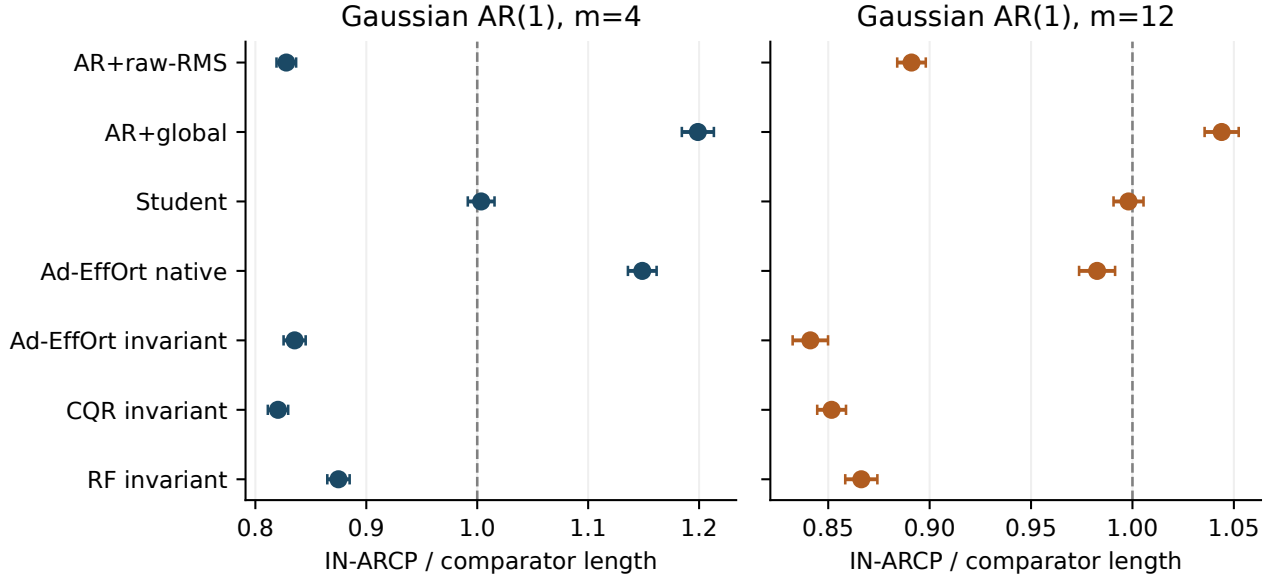
FIGURE 3. Mean-length ratios in the common-Gaussian setting, with paired descriptive 95% Monte Carlo intervals. Ratios below one favor IN-ARCP in mean length. All methods’ coverage estimates are retained in Table 3; these comparisons concern fixed implementations and budgets.
