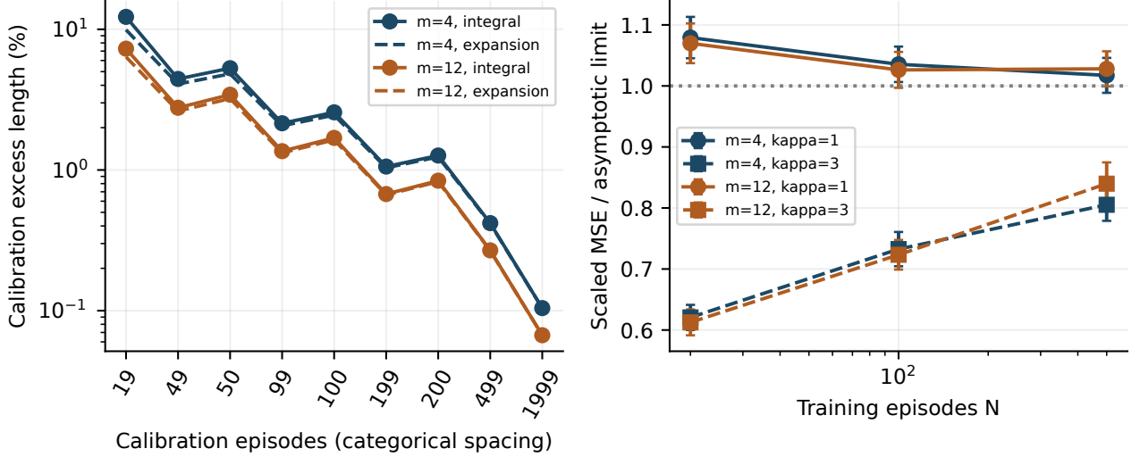
FIGURE 2. Left: known-coefficient finite-calibration excess length and its leading approximation, retaining integer-rank rounding. Adjacent calibration sizes have categorical spacing. Right: empirical scaled coefficient MSE divided by its asymptotic limit; 10,000 fitted samples per point, with 95% Monte Carlo intervals. Stronger amplitude heterogeneity causes a material finite-sample discrepancy.
