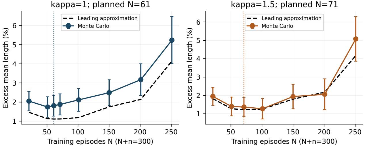
FIGURE 4. Fixed-budget mean-length excess over the Gaussian equivariant oracle. Bars are descriptive 95% Monte Carlo intervals for each mean, not paired differences. Dashed curves show the leading approximation; vertical dotted lines mark prespecified integer planning candidates.
