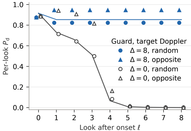
(b) Persistent target, SCR 10 dB
