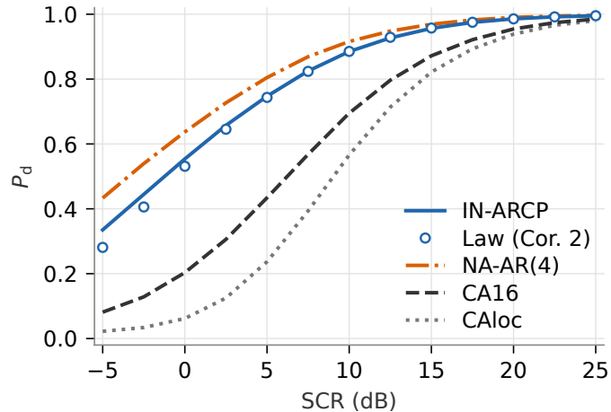
(a) Target in the tested pulse
