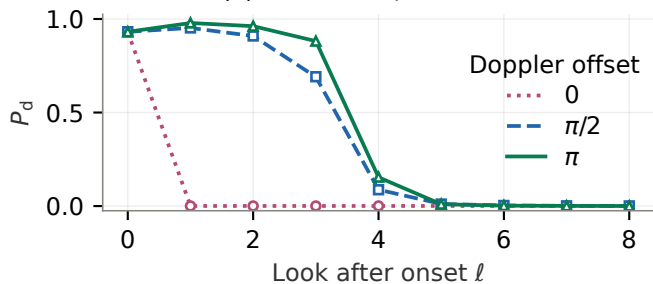
(a) After onset, SCR 10 dB
