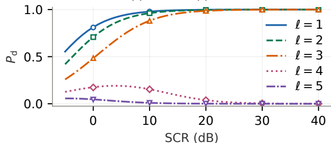
(b) Opposite Doppler, \ell^* = 3.7
