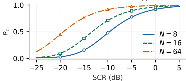
(e) P-ANMF, unknown Doppler
