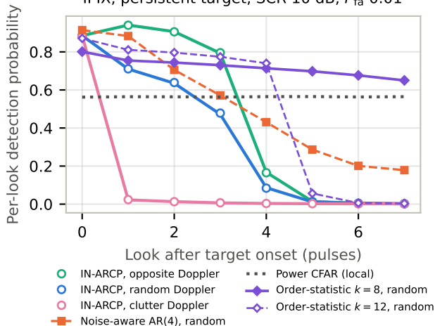
IPIX, persistent target, SCR 10 dB, P_{fa} 0.01
