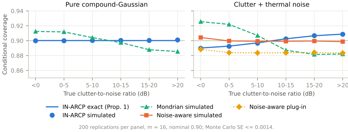
Figure 1: Synthetic verification: coverage conditional on the true clutter-to-noise ratio. The line is the exact law of Proposition 1; markers are simulation.
