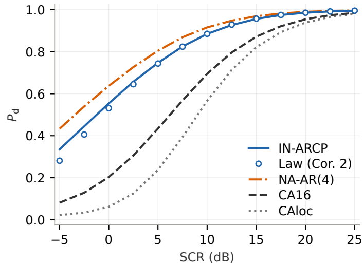
(a) Design P_{fa} = 0.01
