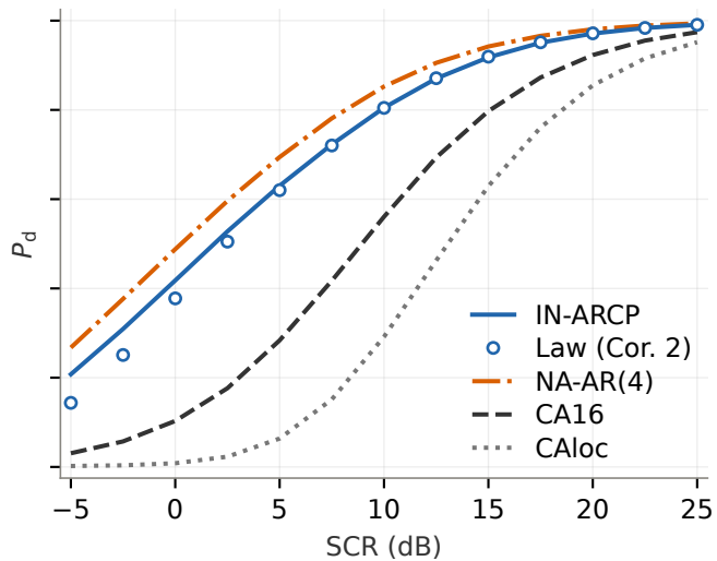
(b) Design P_{fa} = 0.001
