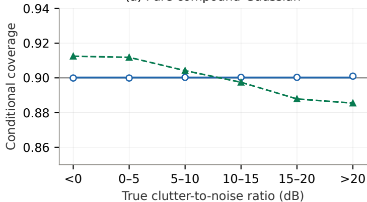
(a) Pure compound-Gaussian
