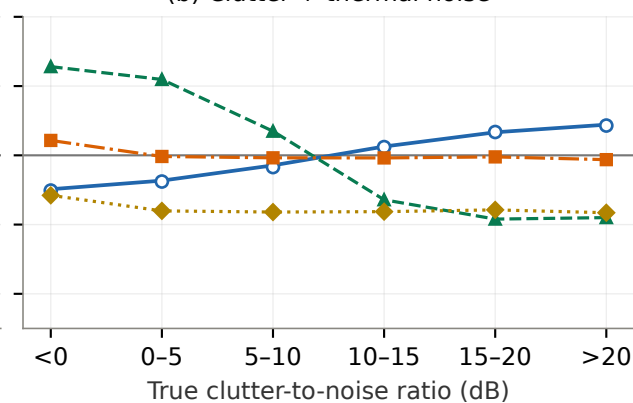
(b) Clutter + thermal noise
