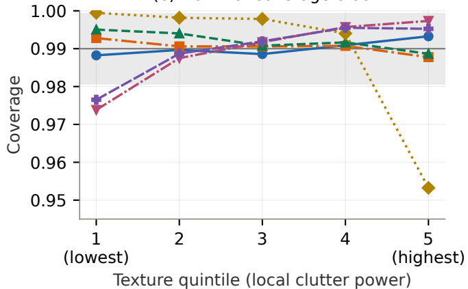
(b) Nominal coverage 0.99
