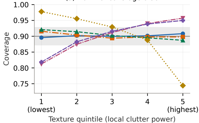
(a) Nominal coverage 0.90
