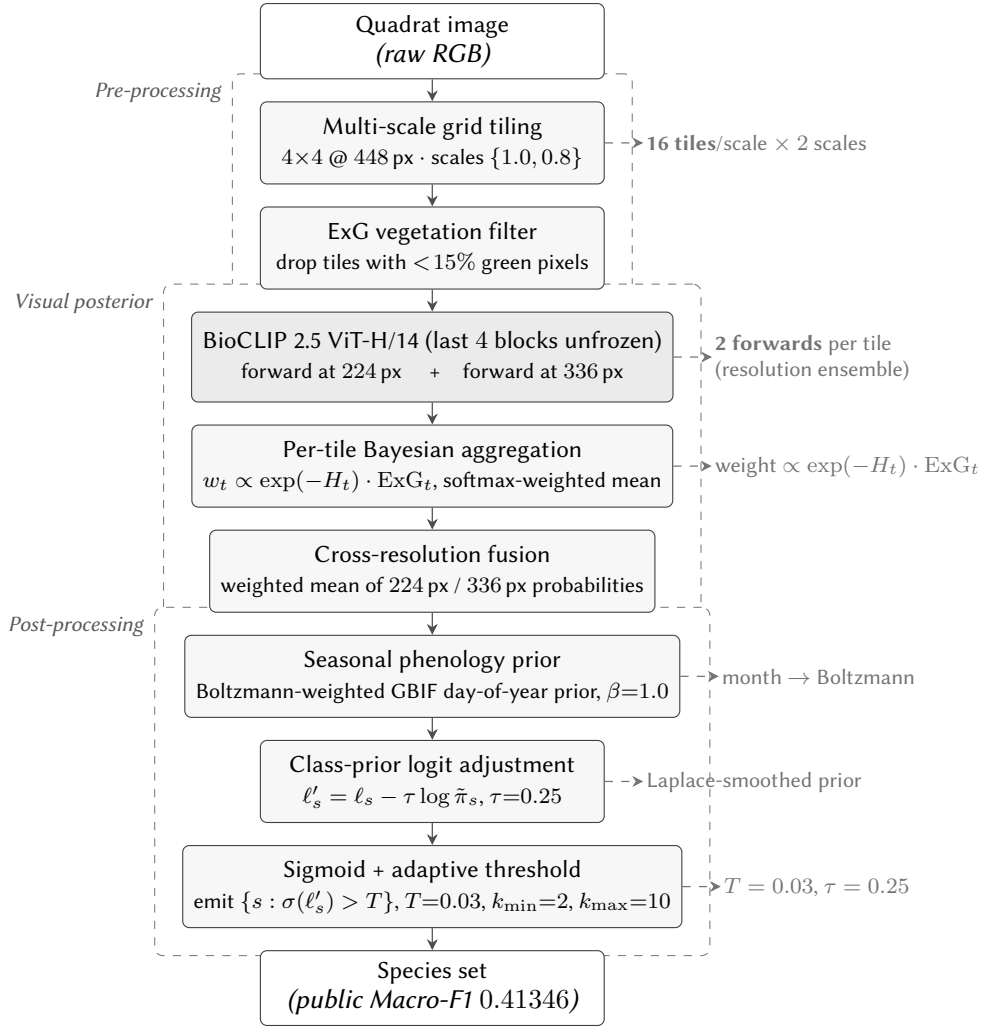
Figure 5: Inference pipeline for the seasonal phenology submission (Pivot 3, public Macro F1 0.41346). Each quadrat is processed at two grid scales (1.0 and 0.8); tiles are screened by an Excess Green (ExG) vegetation filter; the surviving tiles are forwarded through the partially fine-tuned BioCLIP 2.5 ViT-H/14 at two inference resolutions (224 and 336 pixels). Per-tile probabilities are pooled by entropy-weighted Bayesian aggregation, w_t \propto \exp(-H_t) \cdot \text{ExG}_t , and the two resolutions are then averaged. A Boltzmann-weighted seasonal phenology prior over the GBIF day-of-year histogram is added in log space at \beta=1.0 , followed by class-prior logit adjustment ( \tau=0.25 ) and adaptive sigmoid threshold selection ( T=0.03 , k_{\min}=2 , k_{\max}=10 ). The pipeline differs from the anchor (Figure 3) in its multi-scale tiling, ExG screening, and entropy-weighted aggregation; the phenology log-prior is the additional term unique to this submission.
