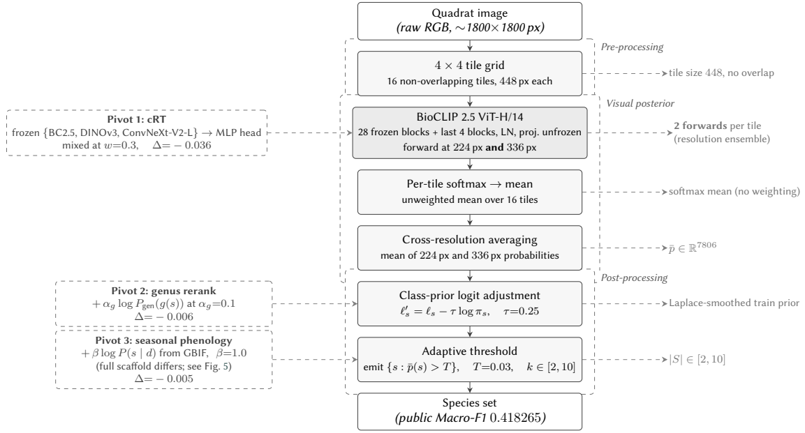
Figure 3: Inference pipeline for the headline anchor submission (solid path; public Macro F1 0.418265). Each quadrat is partitioned into a 4x4 grid of 448-pixel non-overlapping tiles and forwarded through the partially fine-tuned BioCLIP 2.5 ViT-H/14 (lower 28 transformer blocks frozen; last 4 plus LN and projection unfrozen) at two inference resolutions, 224 and 336 pixels. Per-tile softmax probabilities are averaged across the 16 tiles and across the two resolutions, then class-prior logit adjustment ( \tau=0.25 ) is applied before an adaptive sigmoid threshold ( T=0.03 , k_{\min}=2 , k_{\max}=10 ) selects the output species set. Three architecture-orthogonal pivots (dashed; cRT triple-backbone classifier retraining, genus co-occurrence rerank, seasonal phenology prior) indicate where alternative configurations insert into the anchor; all three scored below the anchor on the leaderboard and are reported in Section 4.
