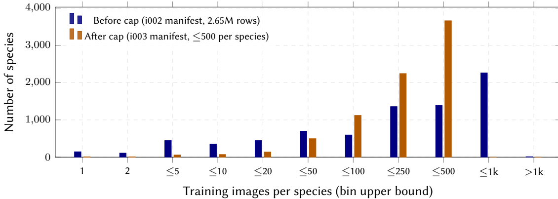
Figure 4: Species count per training-image bin, before and after the i003 per-species cap at 500. The cap collapses the two heaviest bins ( \leq 1k and > 1k ) into the \leq 500 bin and lifts middle bins, but does not move species out of the long tail (left bins). Section 3.3 reports the corresponding leaderboard outcome: this flatter distribution hurt the public Macro F1.
