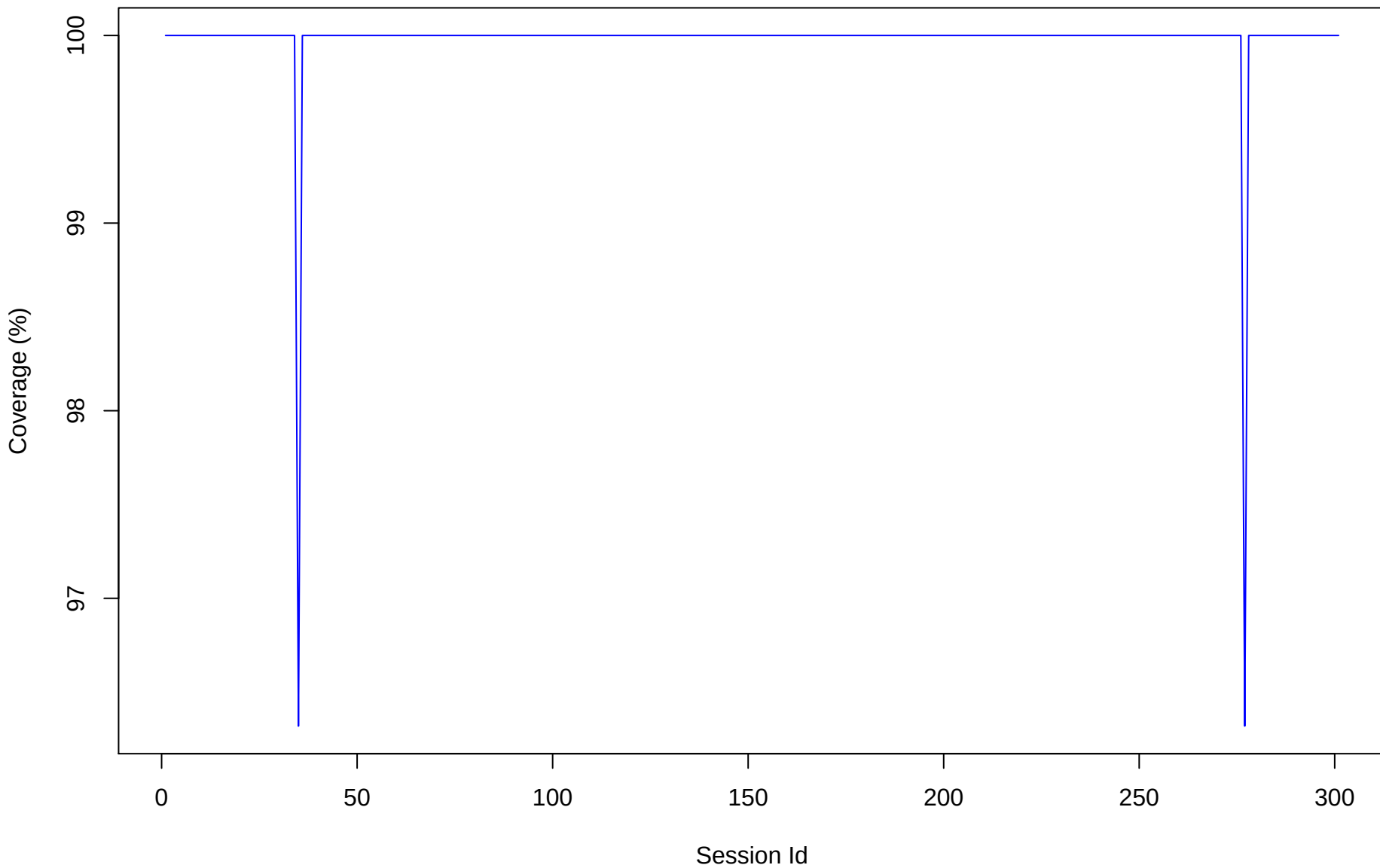
Coverage
