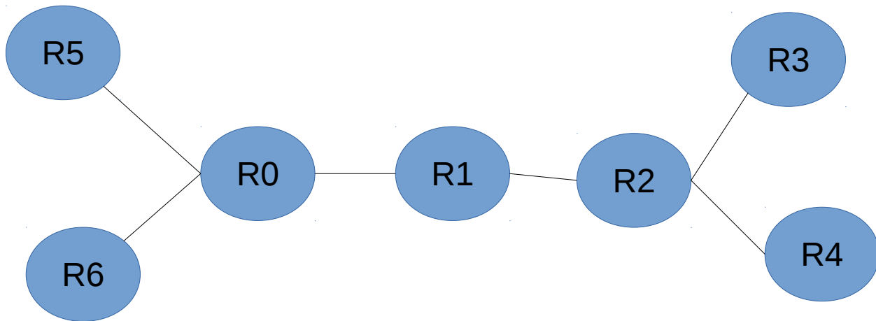
SmallNet
