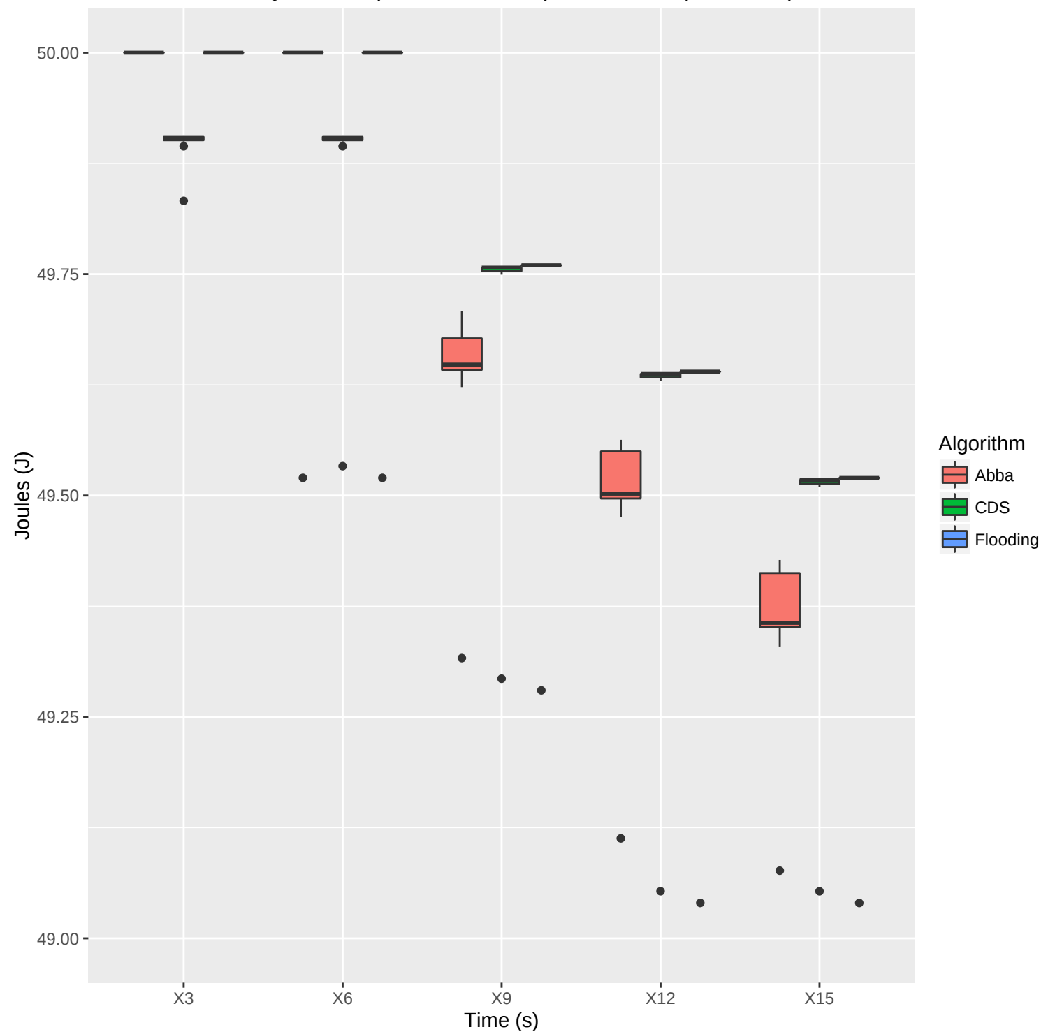
Battery consumption – CDS Paper Network (15 nodes)
