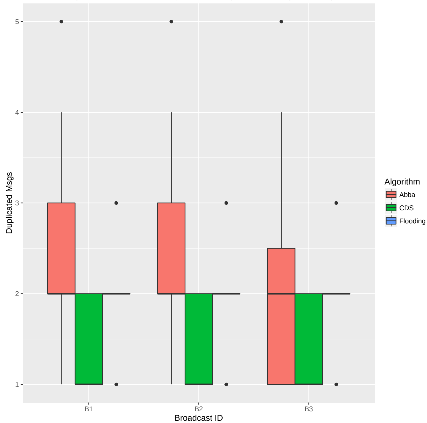
Duplicated Broadcast Msgs – CDS Paper Network (15 nodes)
