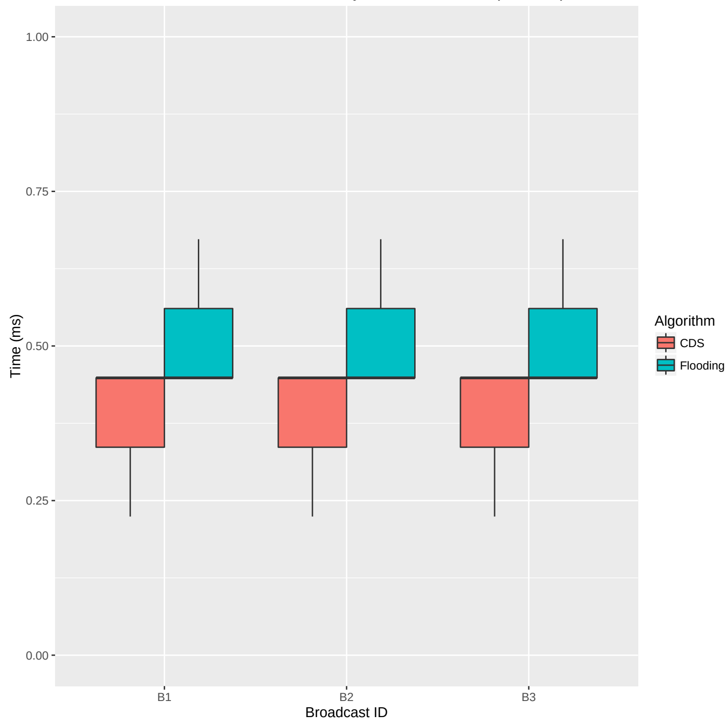
Broadcast Dissemination Delay – Small Network (7 nodes)
