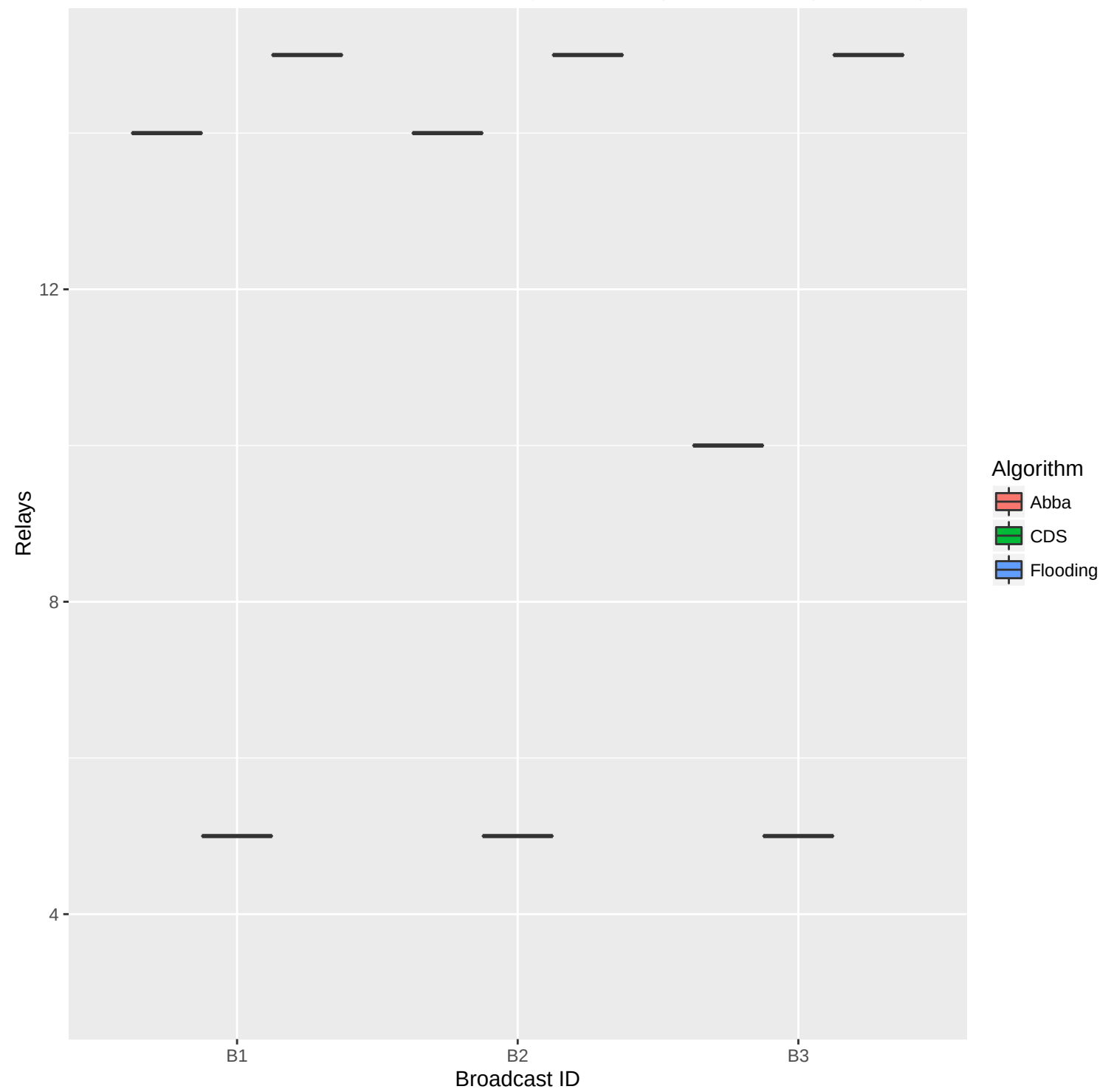
Number Of Relays Per Broadcast Msg – CDS Paper Network (15 nodes)
