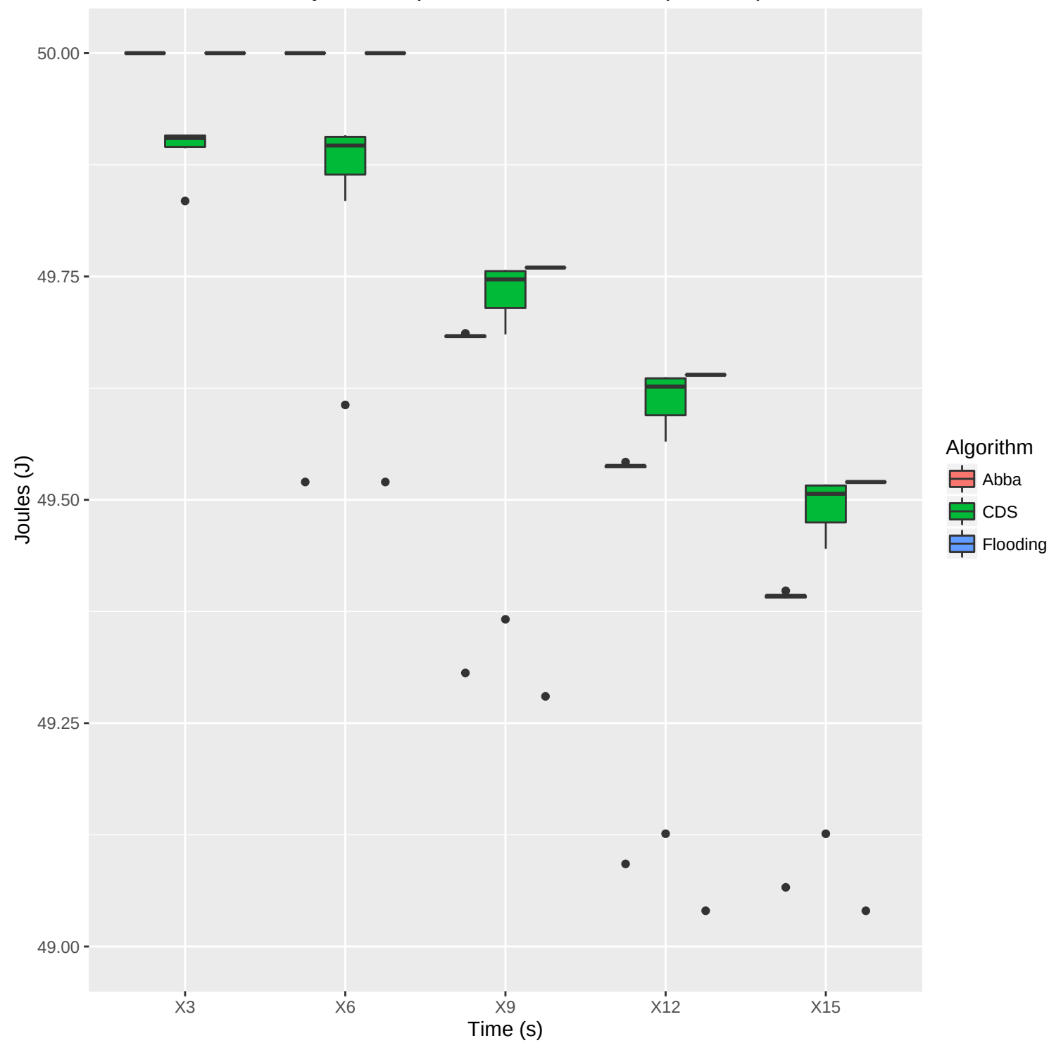
Battery consumption – Small Network (7 nodes)
