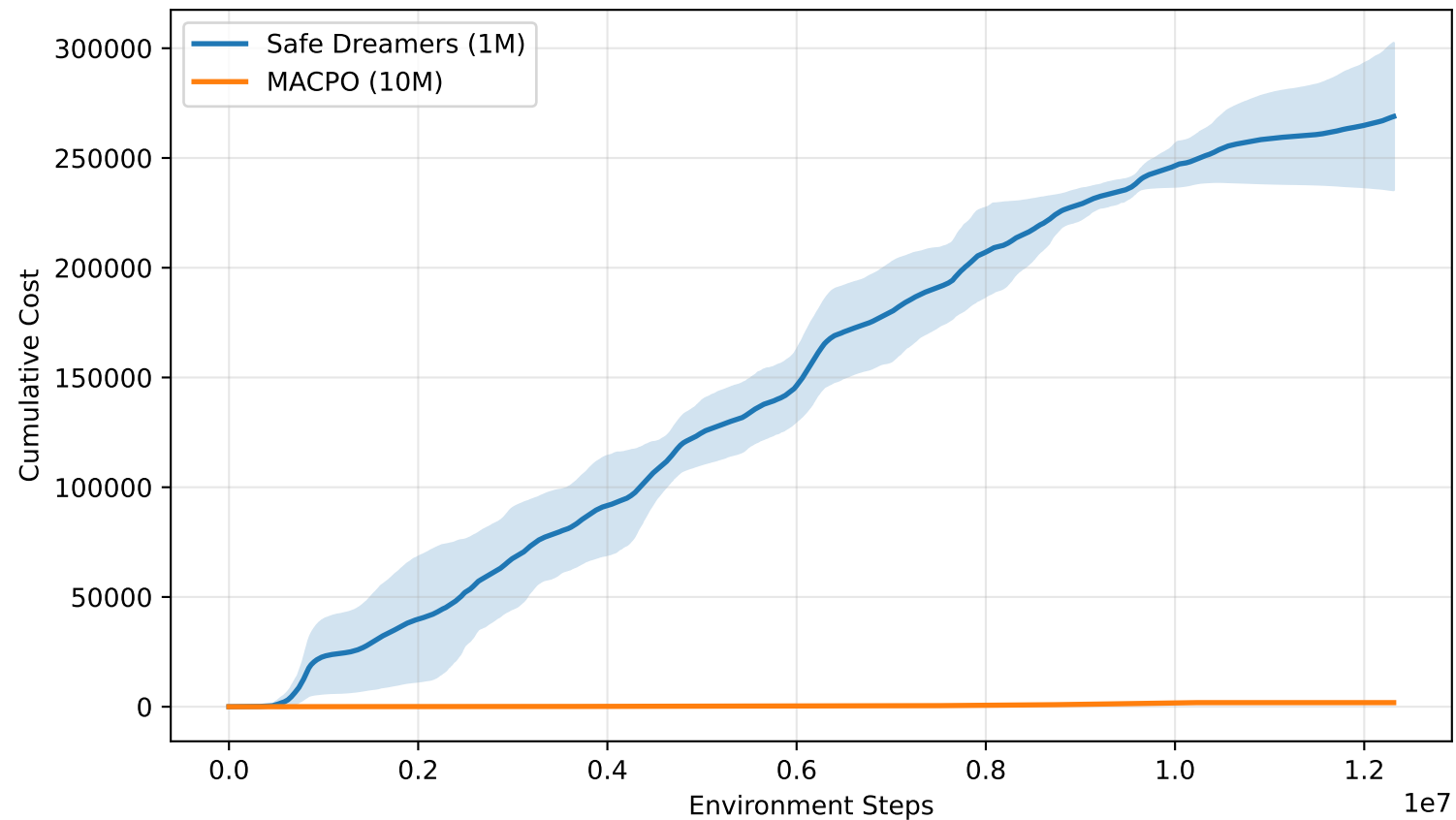
Cumulative Cost — Safety2x4AntVelocity-v0 (d = 25.0)
