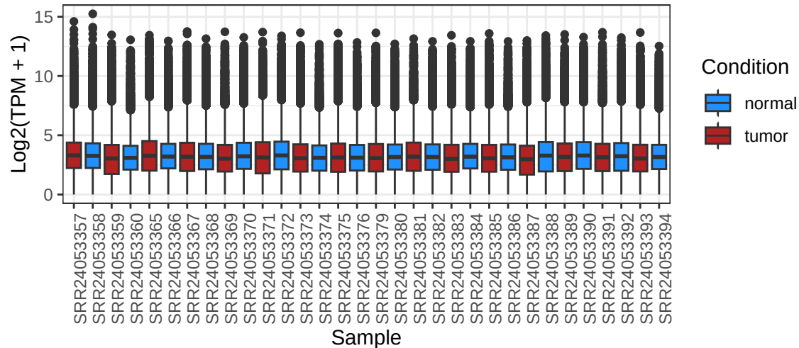
TPM Distribution per Sample
