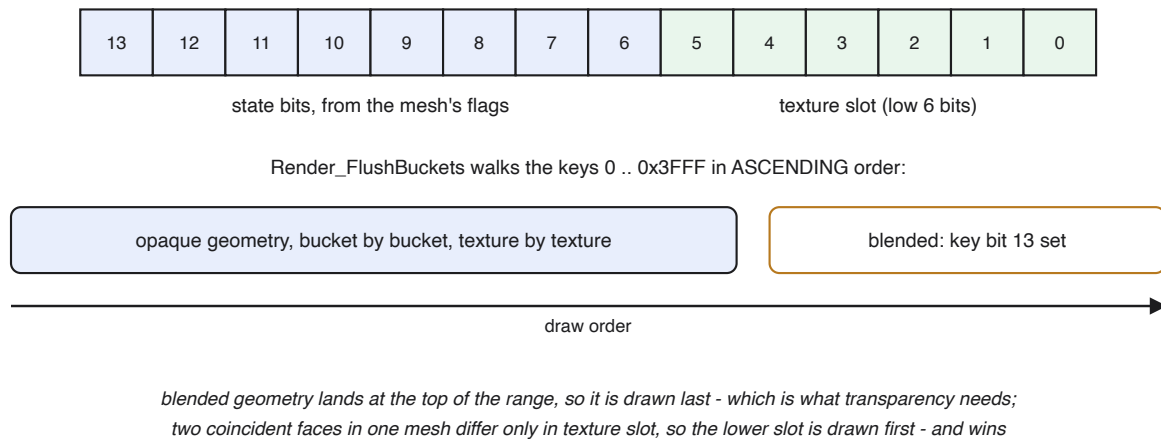
Figure 7 — The draw order is the bucket key, ascending.
