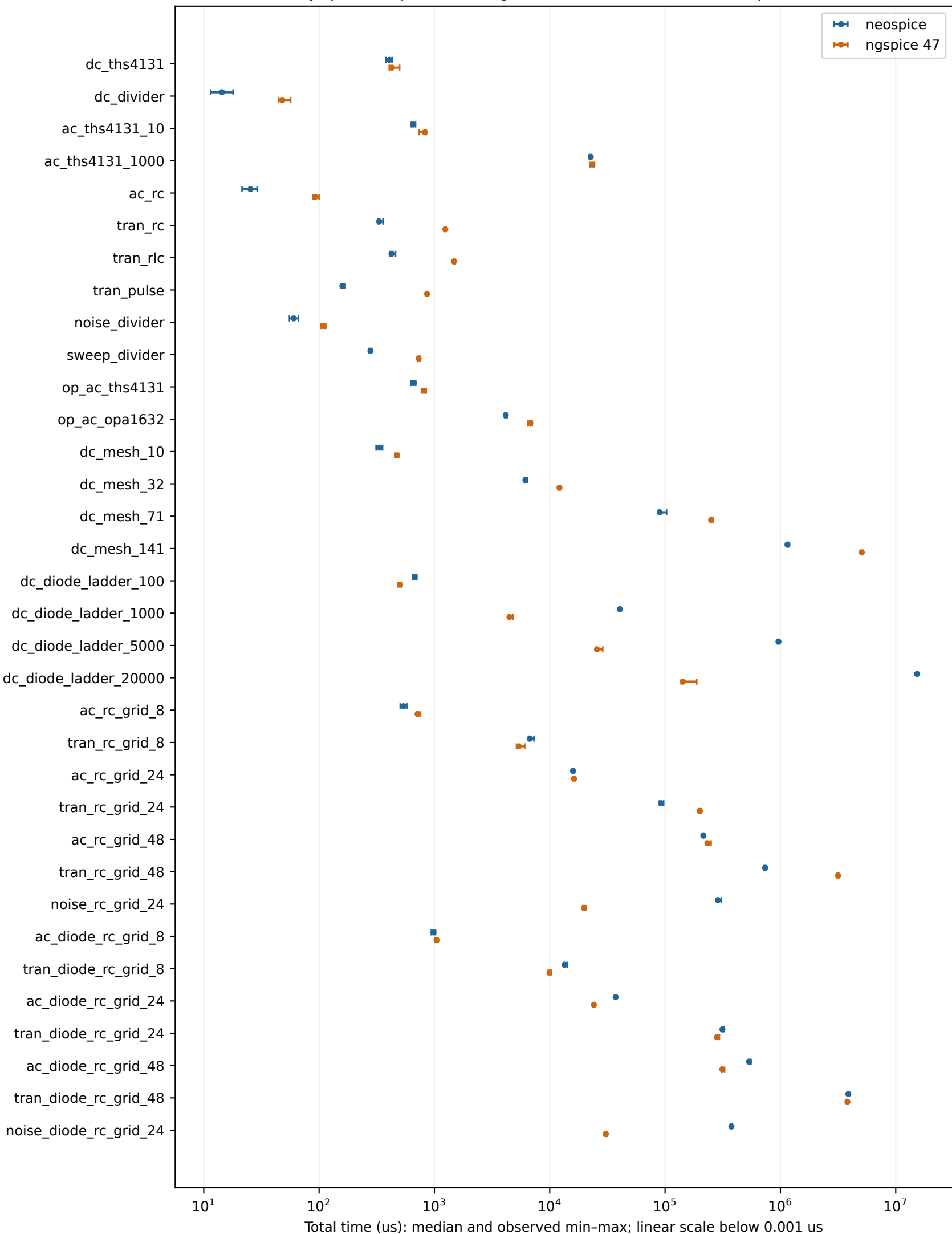
Accuracy-qualified paired timings; failed workloads remain in qualification.csv
