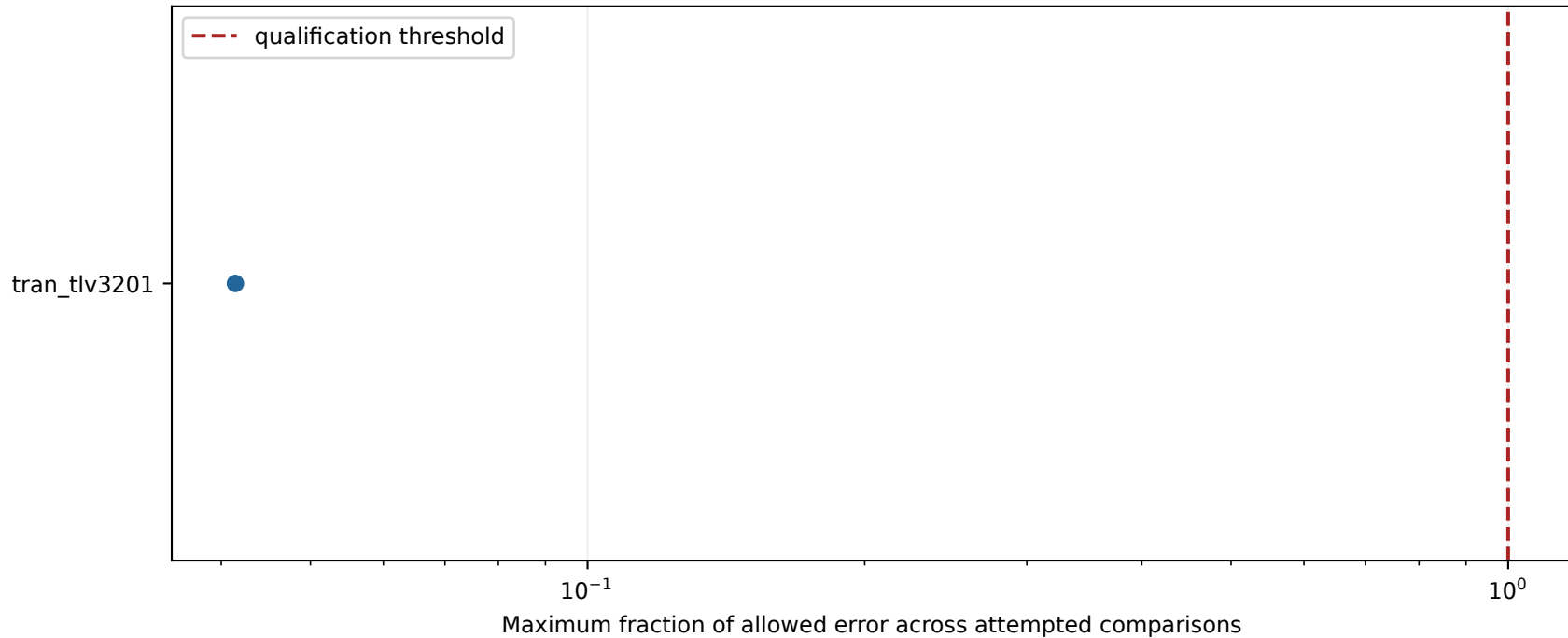
Paired qualification against ngspice 42 (default Sparse, one thread)
