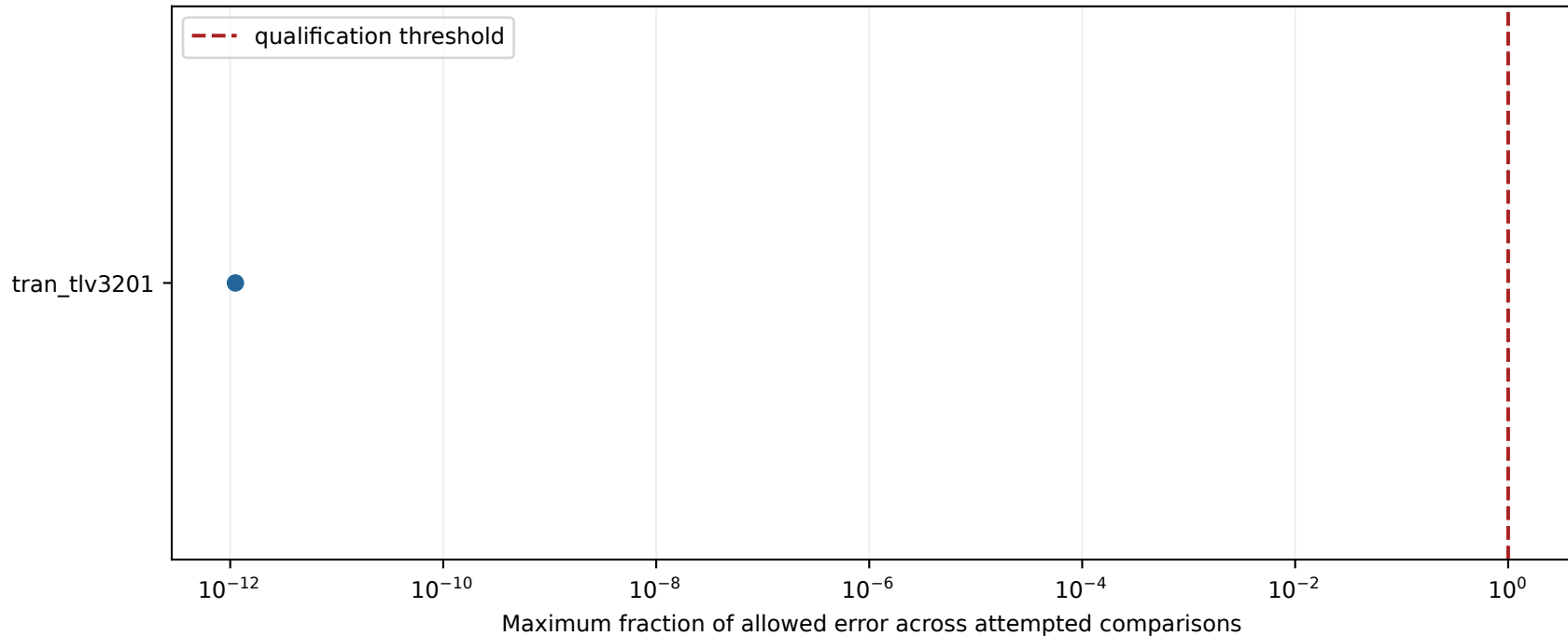
Paired qualification against ngspice 47 (default Sparse, one thread)
