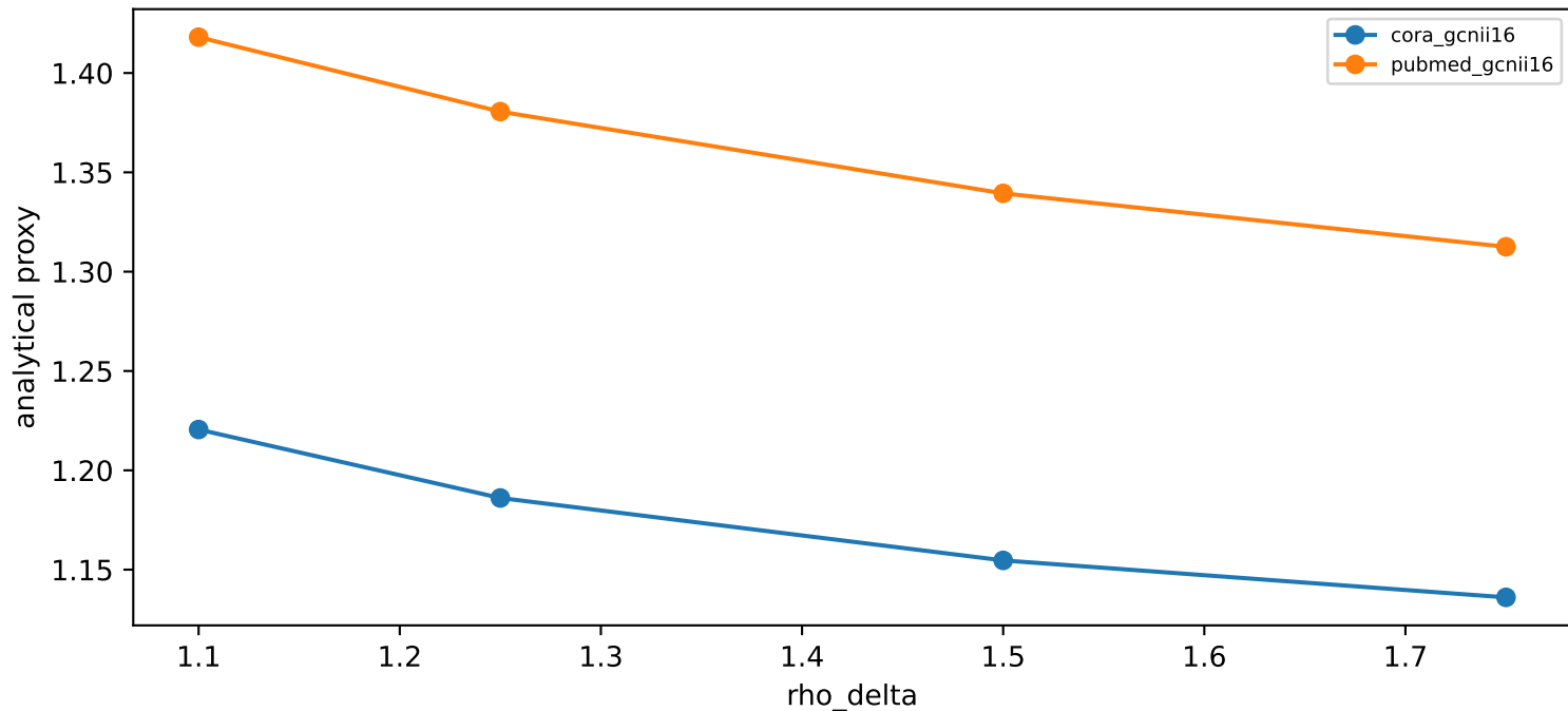
Residual-path sensitivity
