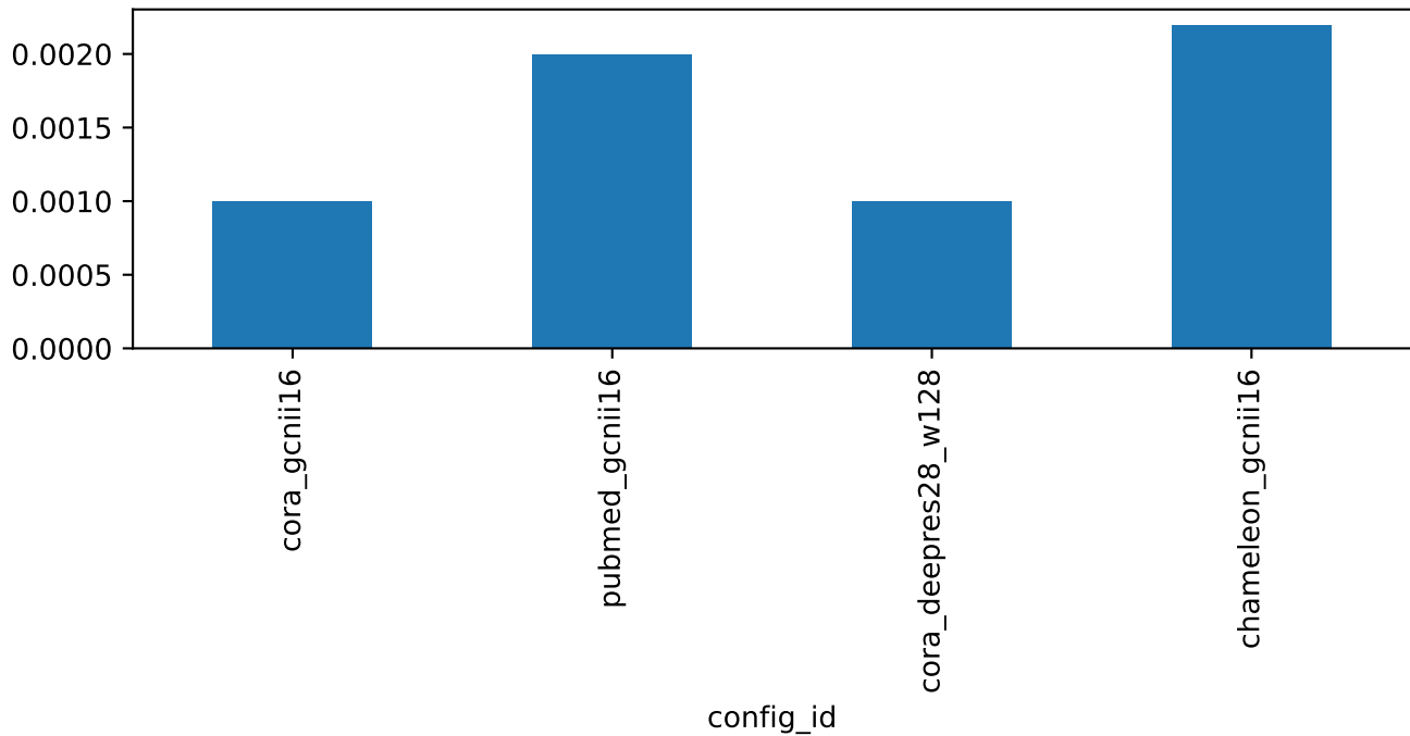
fp8 accuracy
