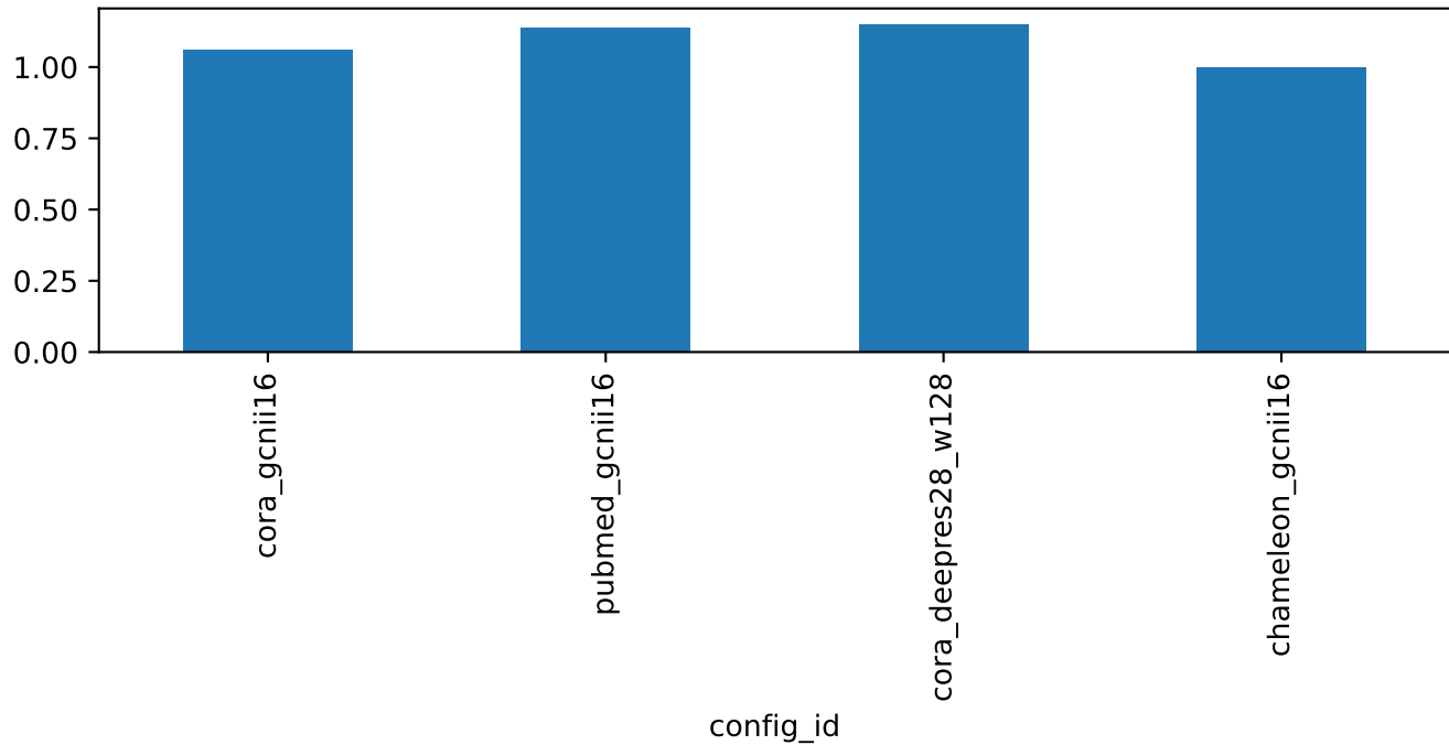
fp8 xorflow speedup
