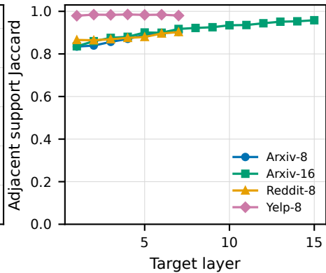
(c) Layerwise persistence
