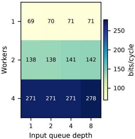
(a) Encoder throughput
