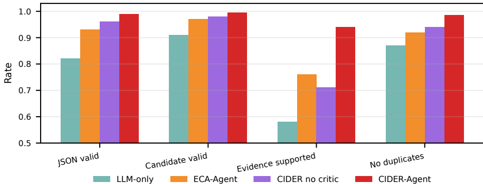
Auditable agent behavior
