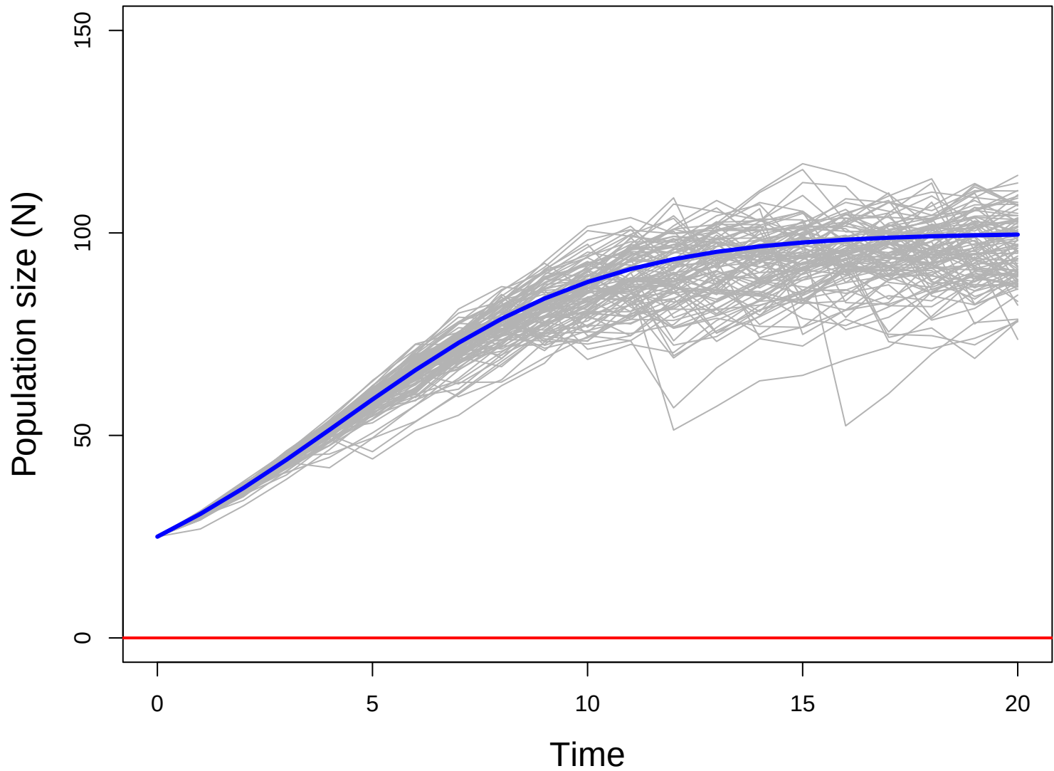
100 Simulations
