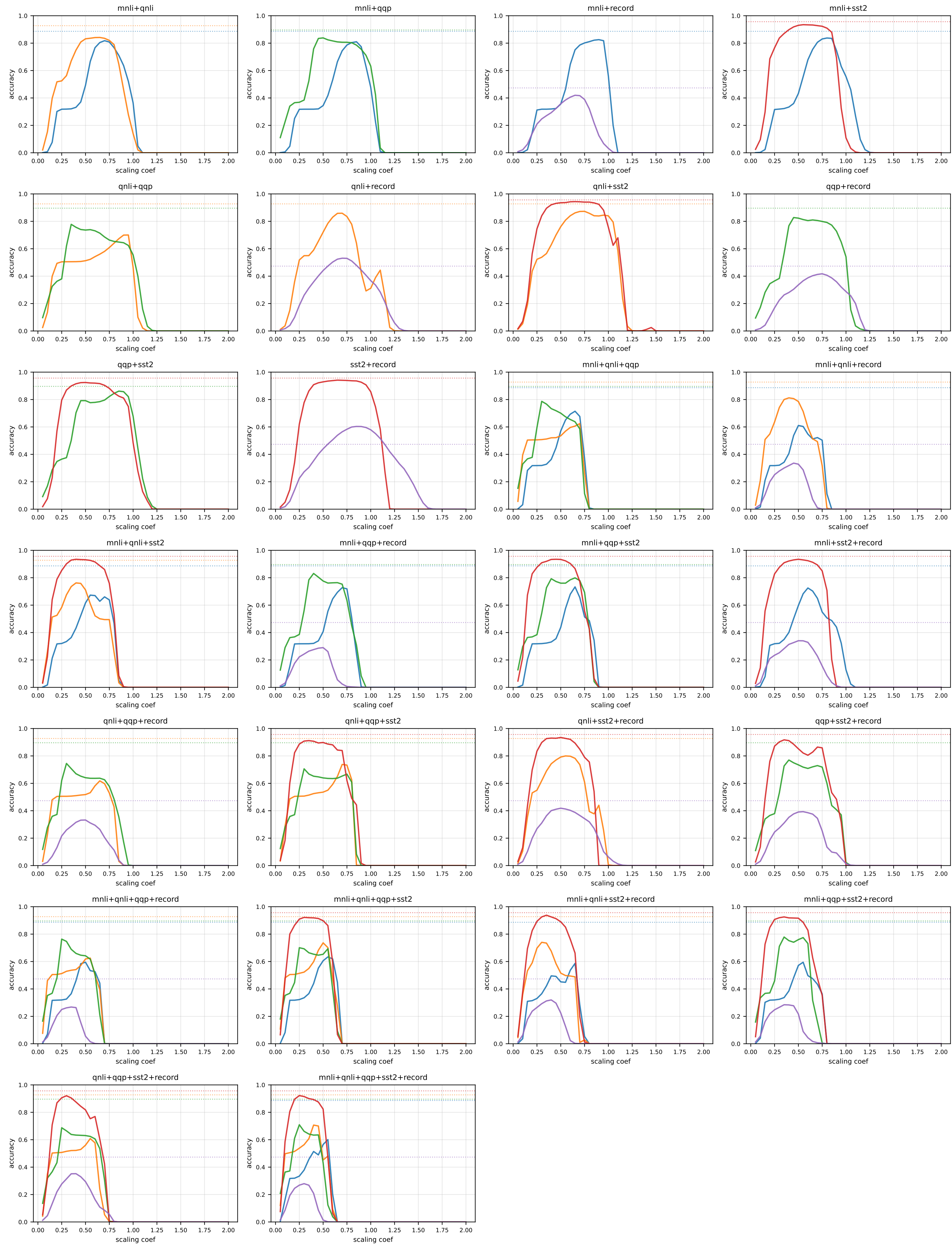
lora: merged accuracy vs scaling coefficient — llama-3.2-1b-instruct (seed 42)
