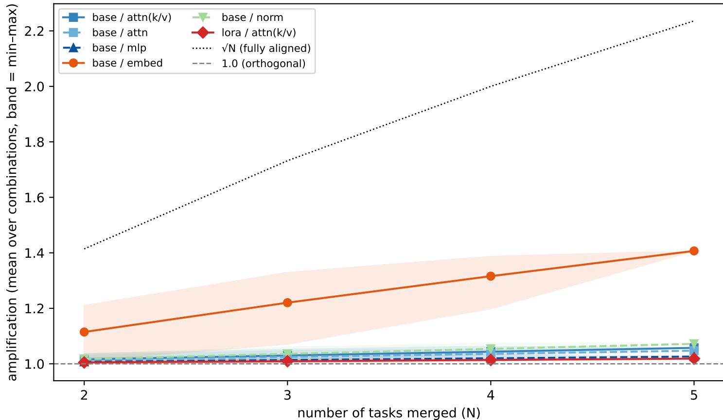
How constructively task vectors add as more tasks are merged
