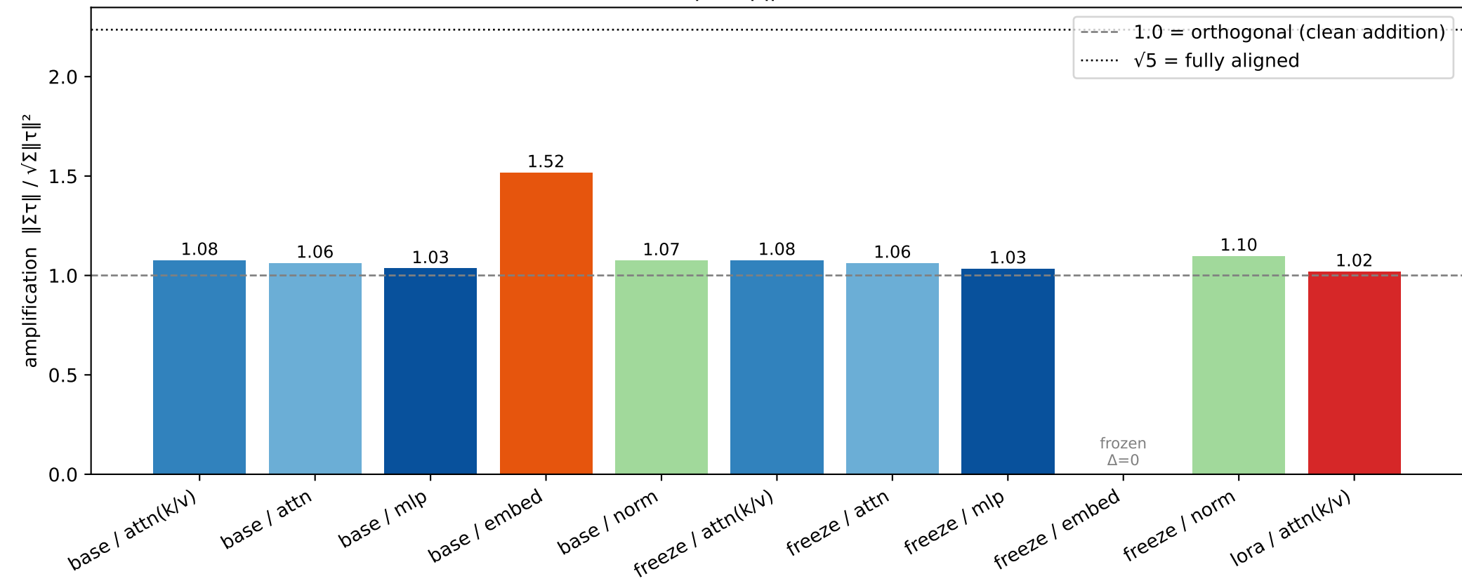
Task-vector amplification, all 5 tasks merged (mnli, qnli, qqp, sst2, record)
