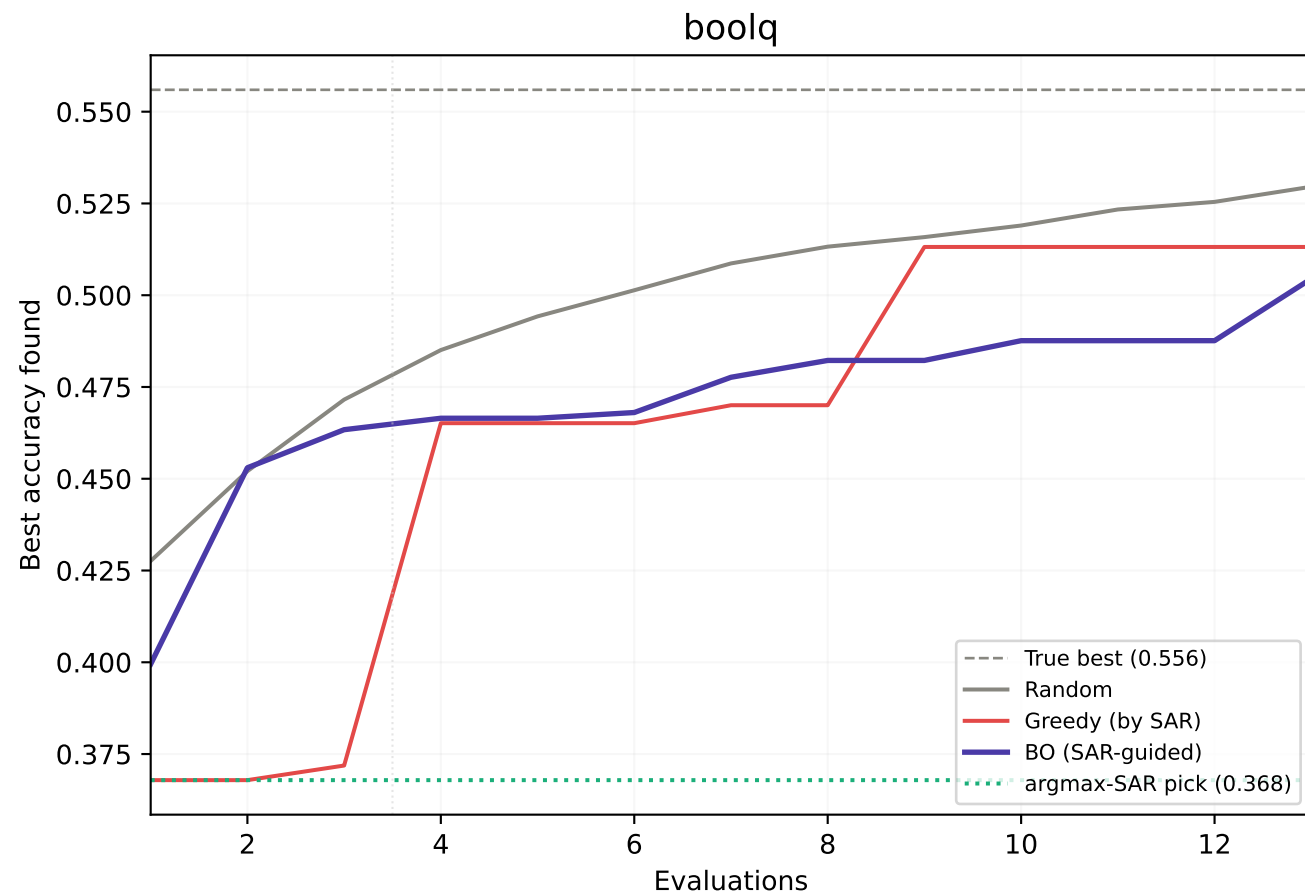
Simulated task selection: BO vs random vs greedy
